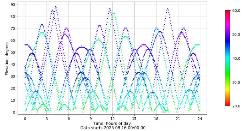
Time-elevation plot for station TALR. Signal to Noise S1C Data file TALR00ESP_R_2023228.xtr
