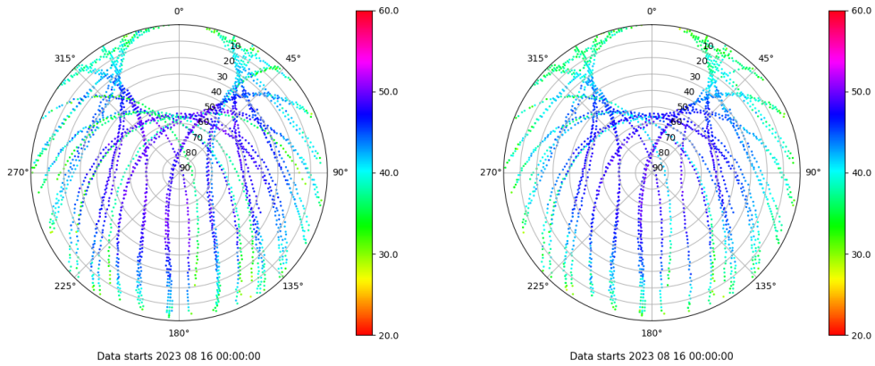
Skyplot for station TALR. Signal to Noise S1C Data file TALR00ESP_R_2023228.xtr Skyplot for station TALR. Signal to Noise S2C Data file TALR00ESP_R_2023228.xtr
