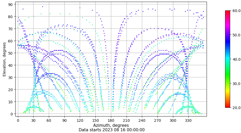
Azimuth-elevation plot for station TALR. Signal to Noise S1C Data file TALR00ESP_R_2023228.xtr
