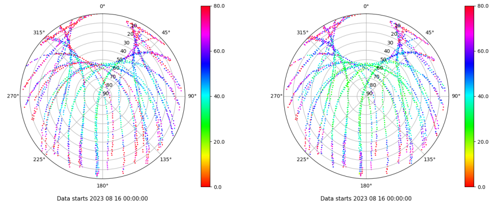
Skyplot for station TALR. Parameter M1C Data file TALR00ESP_R_2023228.xtr Skyplot for station TALR. Parameter M2C Data file TALR00ESP_R_2023228.xtr
