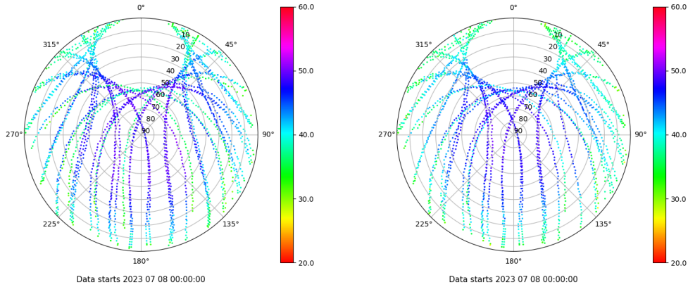
Skyplot for station TALR. Signal to Noise S1C Data file TALR00ESP_R_2023189.xtr Skyplot for station TALR. Signal to Noise S2C Data file TALR00ESP_R_2023189.xtr
