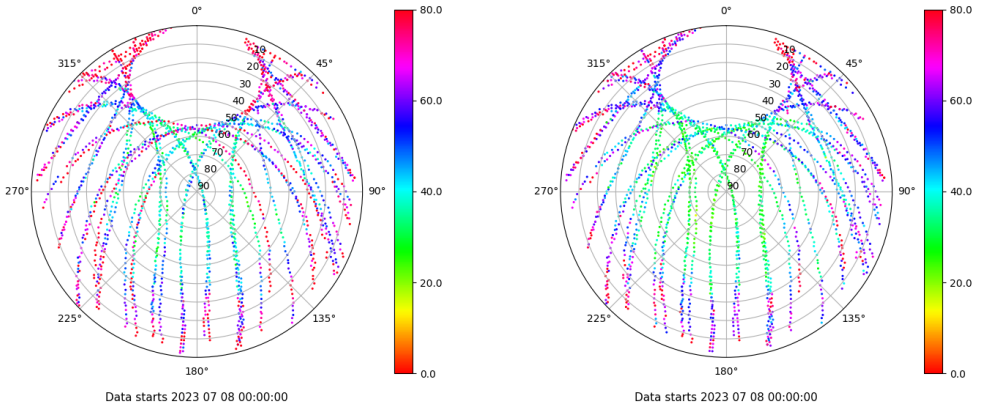
Skyplot for station TALR. Parameter M1C Data file TALR00ESP_R_2023189.xtr Skyplot for station TALR. Parameter M2C Data file TALR00ESP_R_2023189.xtr
