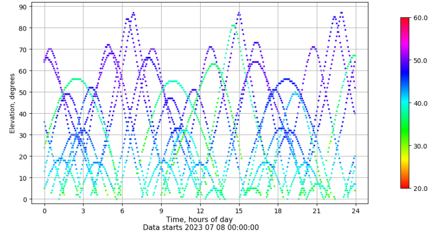
Time-elevation plot for station TALR. Signal to Noise S1C Data file TALR00ESP_R_2023189.xtr
