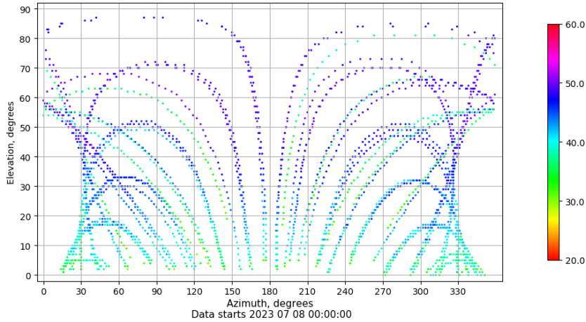
Azimuth-elevation plot for station TALR. Signal to Noise S1C Data file TALR00ESP_R_2023189.xtr
