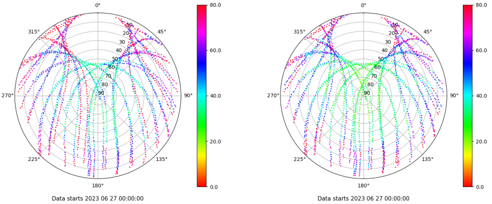
Skyplot for station TALR. Parameter M1C Data file TALR00ESP_R_2023178.xtr Skyplot for station TALR. Parameter M2C Data file TALR00ESP_R_2023178.xtr
