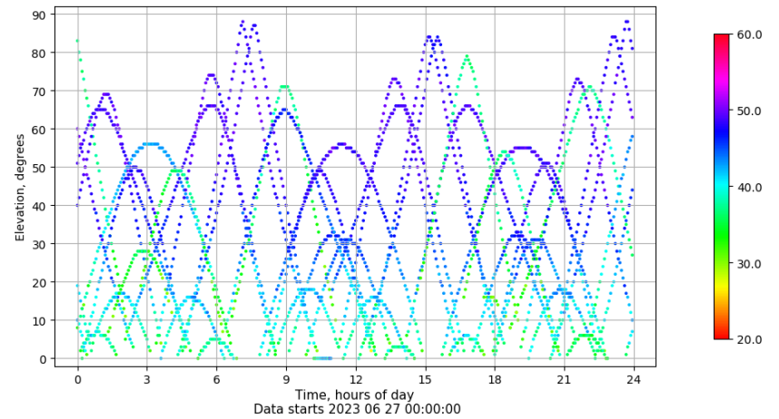
Time-elevation plot for station TALR. Signal to Noise S1C Data file TALR00ESP_R_2023178.xtr
