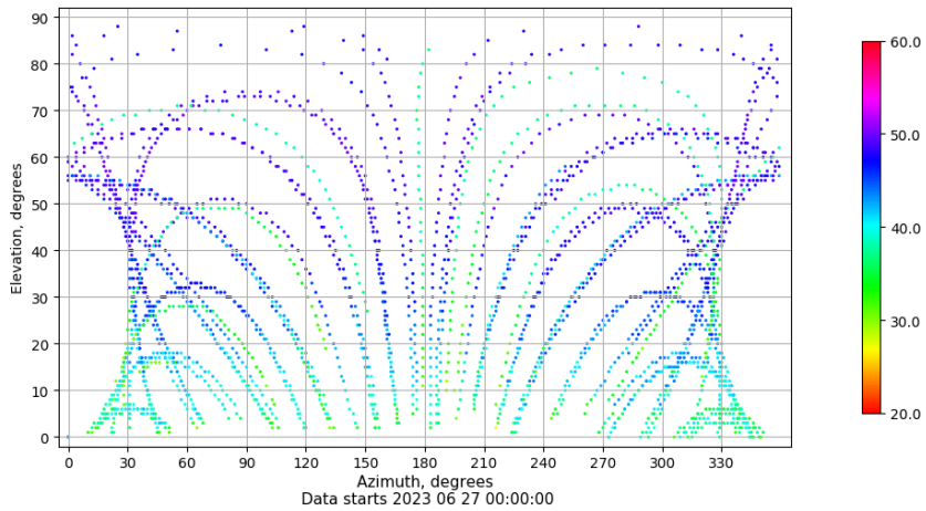
Azimuth-elevation plot for station TALR. Signal to Noise S1C Data file TALR00ESP_R_2023178.xtr
