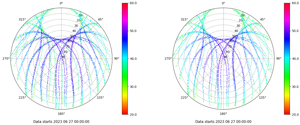
Skyplot for station TALR. Signal to Noise S1C Data file TALR00ESP_R_2023178.xtr Skyplot for station TALR. Signal to Noise S2C Data file TALR00ESP_R_2023178.xtr
