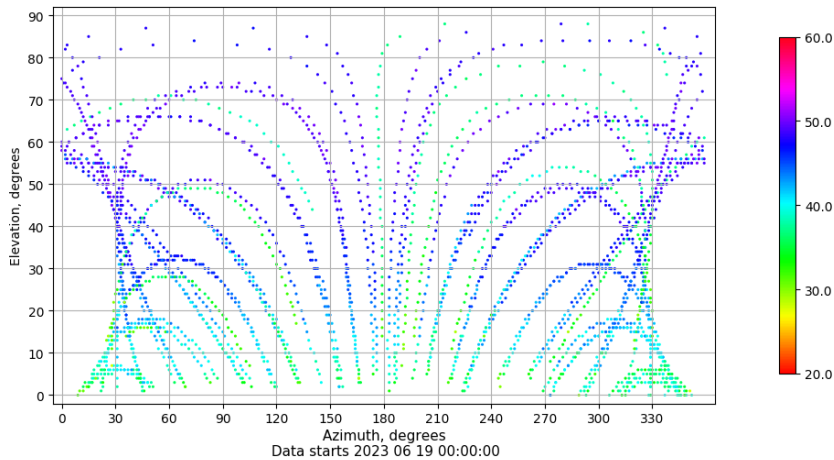
Azimuth-elevation plot for station TALR. Signal to Noise S1C Data file TALR00ESP_R_2023170.xtr
