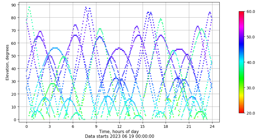
Time-elevation plot for station TALR. Signal to Noise S1C Data file TALR00ESP_R_2023170.xtr
