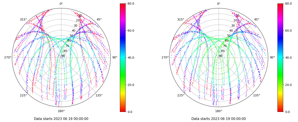
Skyplot for station TALR. Parameter M1C Data file TALR00ESP_R_2023170.xtr Skyplot for station TALR. Parameter M2C Data file TALR00ESP_R_2023170.xtr
