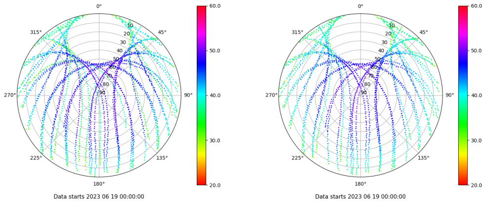
Skyplot for station TALR. Signal to Noise S1C Data file TALR00ESP_R_2023170.xtr Skyplot for station TALR. Signal to Noise S2C Data file TALR00ESP_R_2023170.xtr
