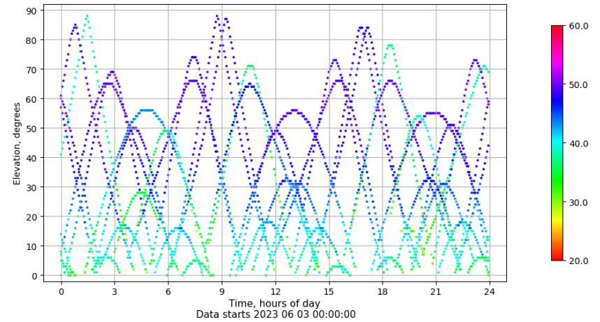
Time-elevation plot for station TALR. Signal to Noise S1C Data file TALR00ESP_R_2023154.xtr
