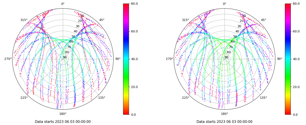
Skyplot for station TALR. Parameter M1C Data file TALR00ESP_R_2023154.xtr Skyplot for station TALR. Parameter M2C Data file TALR00ESP_R_2023154.xtr
