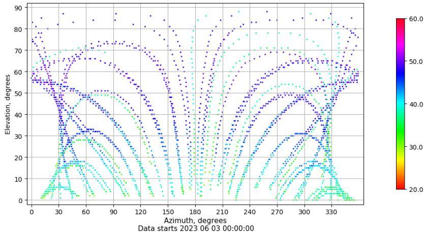
Azimuth-elevation plot for station TALR. Signal to Noise S1C Data file TALR00ESP_R_2023154.xtr
