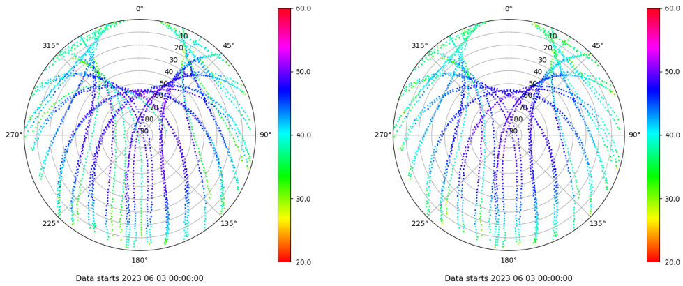
Skyplot for station TALR. Signal to Noise S1C Data file TALR00ESP_R_2023154.xtr Skyplot for station TALR. Signal to Noise S2C Data file TALR00ESP_R_2023154.xtr
