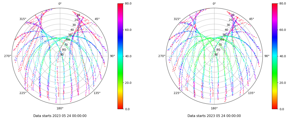
Skyplot for station TALR. Parameter M1C Data file TALR00ESP_R_2023144.xtr Skyplot for station TALR. Parameter M2C Data file TALR00ESP_R_2023144.xtr
