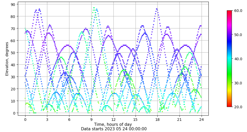
Time-elevation plot for station TALR. Signal to Noise S1C Data file TALR00ESP_R_2023144.xtr
