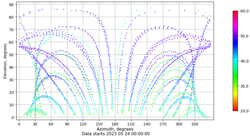
Azimuth-elevation plot for station TALR. Signal to Noise S1C Data file TALR00ESP_R_2023144.xtr
