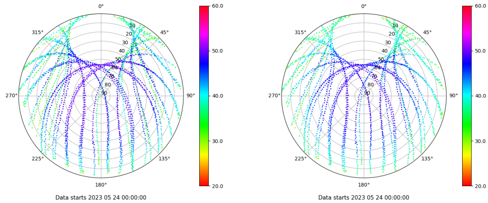
Skyplot for station TALR. Signal to Noise S1C Data file TALR00ESP_R_2023144.xtr Skyplot for station TALR. Signal to Noise S2C Data file TALR00ESP_R_2023144.xtr
