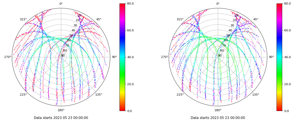
Skyplot for station TALR. Parameter M1C Data file TALR00ESP_R_2023143.xtr Skyplot for station TALR. Parameter M2C Data file TALR00ESP_R_2023143.xtr
