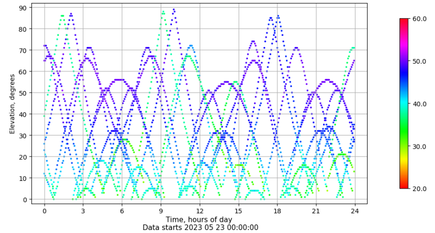
Time-elevation plot for station TALR. Signal to Noise S1C Data file TALR00ESP_R_2023143.xtr
