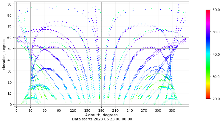
Azimuth-elevation plot for station TALR. Signal to Noise S1C Data file TALR00ESP_R_2023143.xtr
