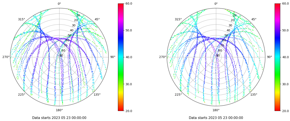
Skyplot for station TALR. Signal to Noise S1C Data file TALR00ESP_R_2023143.xtr Skyplot for station TALR. Signal to Noise S2C Data file TALR00ESP_R_2023143.xtr
