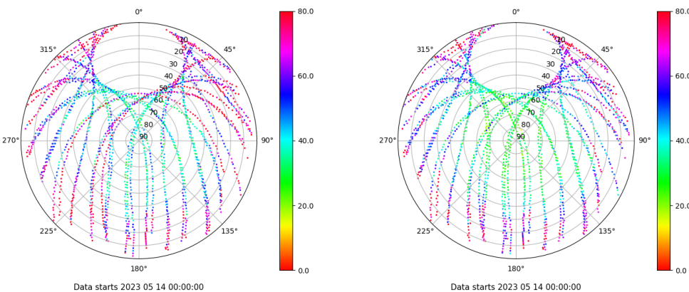
Skyplot for station TALR. Parameter M1C Data file TALR00ESP_R_2023134.xtr Skyplot for station TALR. Parameter M2C Data file TALR00ESP_R_2023134.xtr
