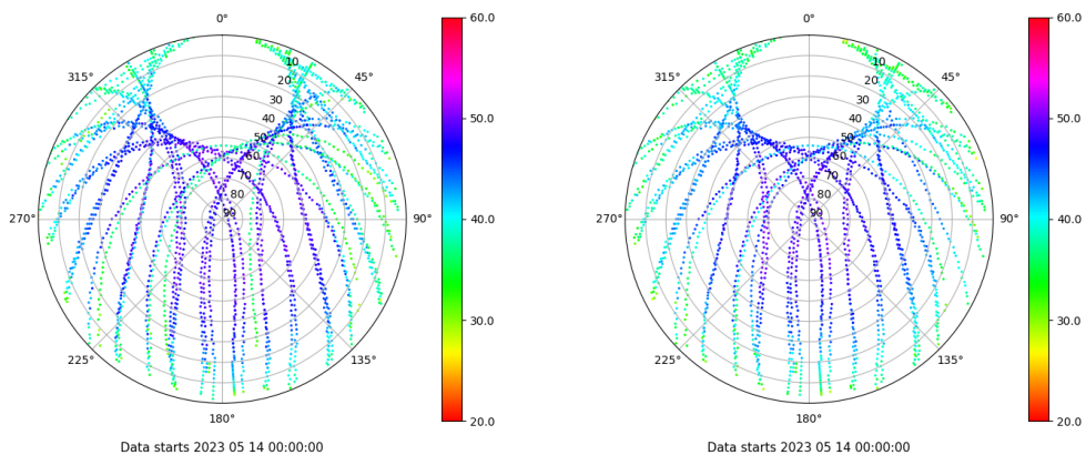
Skyplot for station TALR. Signal to Noise S1C Data file TALR00ESP_R_2023134.xtr Skyplot for station TALR. Signal to Noise S2C Data file TALR00ESP_R_2023134.xtr
