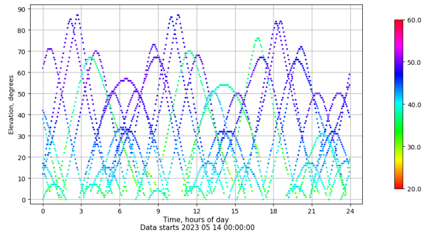
Time-elevation plot for station TALR. Signal to Noise S1C Data file TALR00ESP_R_2023134.xtr
