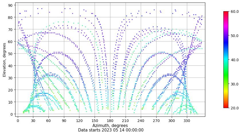
Azimuth-elevation plot for station TALR. Signal to Noise S1C Data file TALR00ESP_R_2023134.xtr
