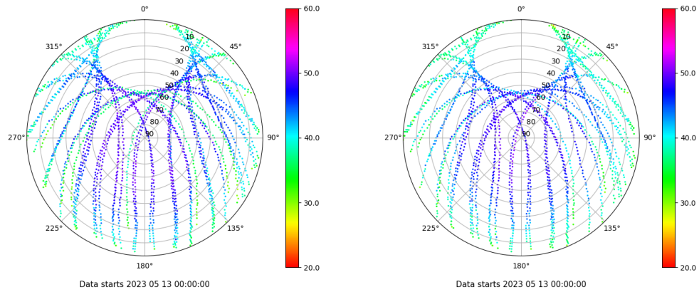
Skyplot for station TALR. Signal to Noise S1C Data file TALR00ESP_R_2023133.xtr Skyplot for station TALR. Signal to Noise S2C Data file TALR00ESP_R_2023133.xtr
