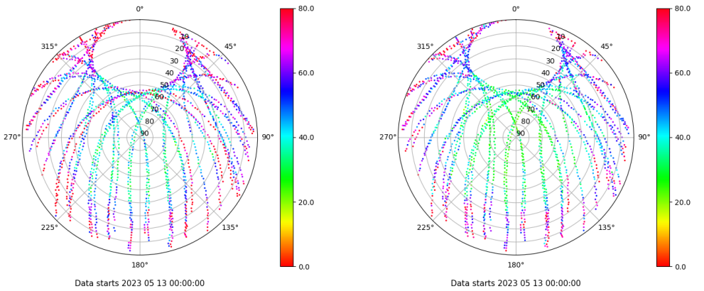
Skyplot for station TALR. Parameter M1C Data file TALR00ESP_R_2023133.xtr Skyplot for station TALR. Parameter M2C Data file TALR00ESP_R_2023133.xtr
