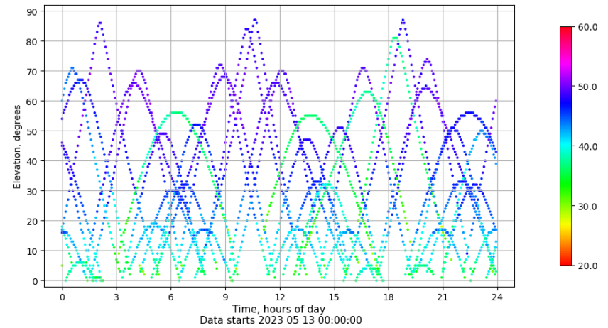
Time-elevation plot for station TALR. Signal to Noise S1C Data file TALR00ESP_R_2023133.xtr
