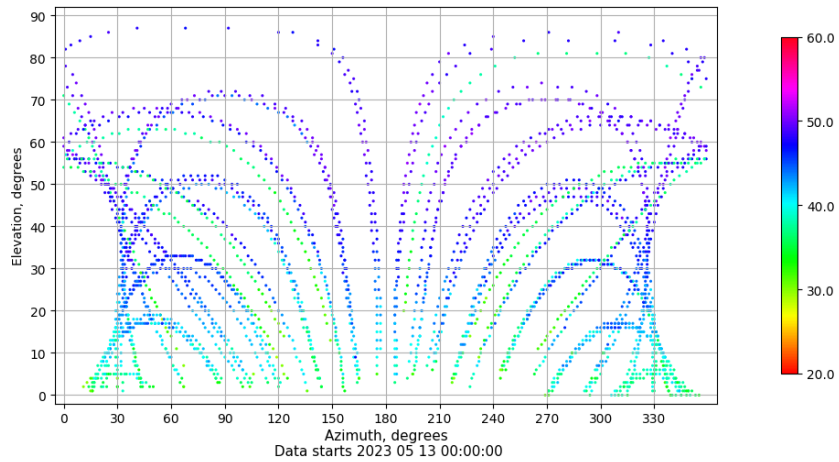
Azimuth-elevation plot for station TALR. Signal to Noise S1C Data file TALR00ESP_R_2023133.xtr
