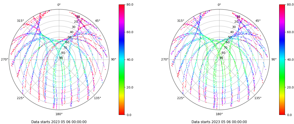
Skyplot for station TALR. Parameter M1C Data file TALR00ESP_R_2023126.xtr Skyplot for station TALR. Parameter M2C Data file TALR00ESP_R_2023126.xtr
