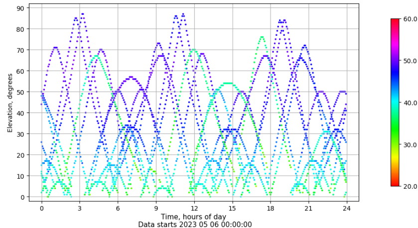
Time-elevation plot for station TALR. Signal to Noise S1C Data file TALR00ESP_R_2023126.xtr
