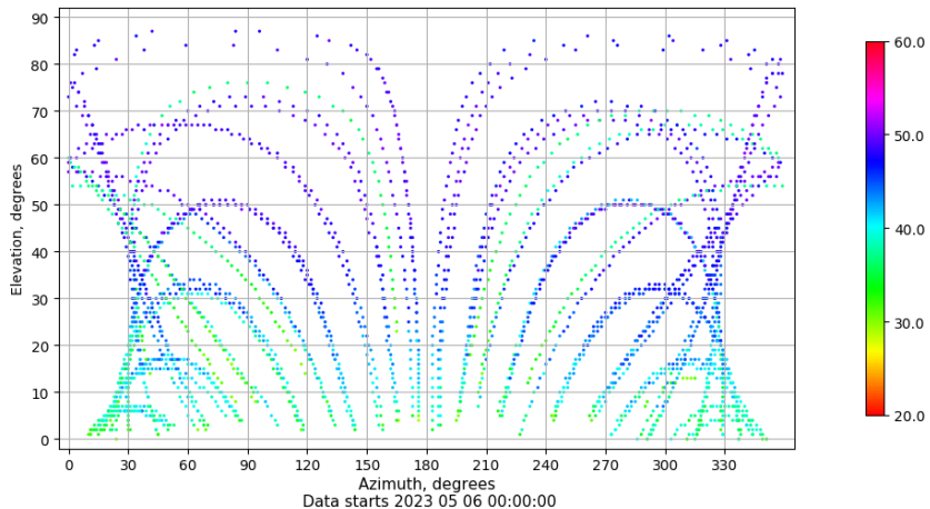
Azimuth-elevation plot for station TALR. Signal to Noise S1C Data file TALR00ESP_R_2023126.xtr
