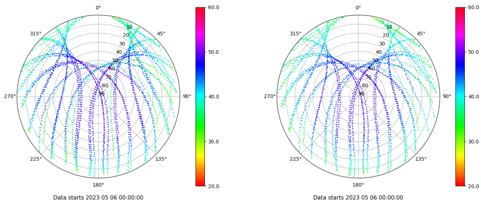
Skyplot for station TALR. Signal to Noise S1C Data file TALR00ESP_R_2023126.xtr Skyplot for station TALR. Signal to Noise S2C Data file TALR00ESP_R_2023126.xtr
