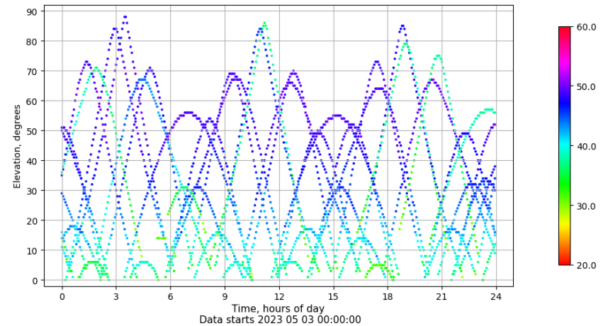
Time-elevation plot for station TALR. Signal to Noise S1C Data file TALR00ESP_R_2023123.xtr
