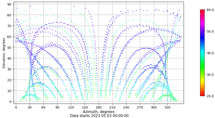
Azimuth-elevation plot for station TALR. Signal to Noise S1C Data file TALR00ESP_R_2023123.xtr
