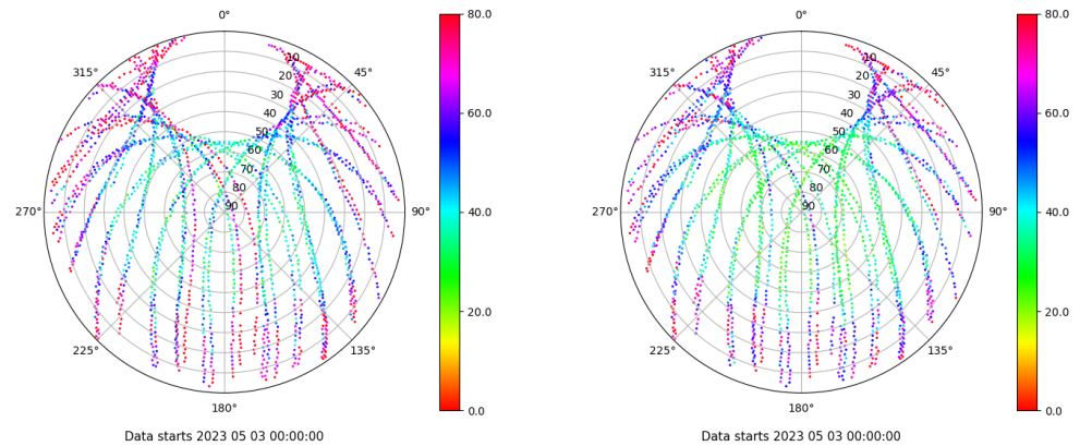
Skyplot for station TALR. Parameter M1C Data file TALR00ESP_R_2023123.xtr Skyplot for station TALR. Parameter M2C Data file TALR00ESP_R_2023123.xtr
