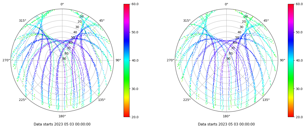
Skyplot for station TALR. Signal to Noise S1C Data file TALR00ESP_R_2023123.xtr Skyplot for station TALR. Signal to Noise S2C Data file TALR00ESP_R_2023123.xtr
