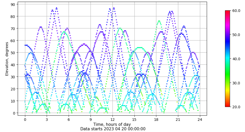
Time-elevation plot for station TALR. Signal to Noise S1C Data file TALR00ESP_R_2023110.xtr
