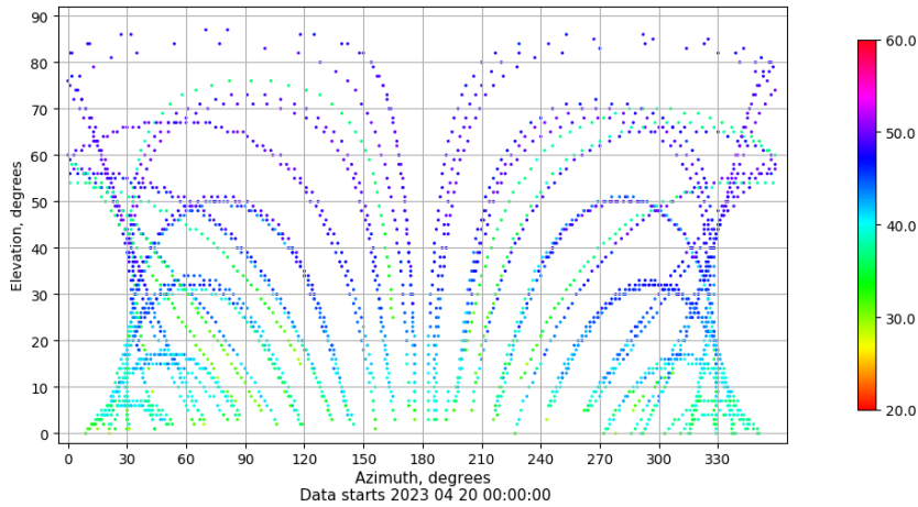
Azimuth-elevation plot for station TALR. Signal to Noise S1C Data file TALR00ESP_R_2023110.xtr
