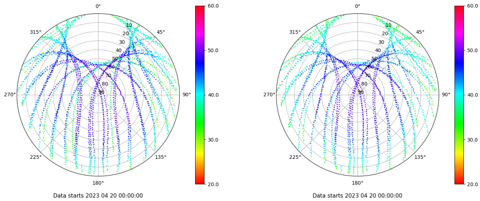
Skyplot for station TALR. Signal to Noise S1C Data file TALR00ESP_R_2023110.xtr Skyplot for station TALR. Signal to Noise S2C Data file TALR00ESP_R_2023110.xtr
