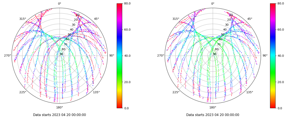
Skyplot for station TALR. Parameter M1C Data file TALR00ESP_R_2023110.xtr Skyplot for station TALR. Parameter M2C Data file TALR00ESP_R_2023110.xtr
