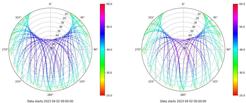
Skyplot for station TALR. Signal to Noise S1C Data file TALR00ESP_R_2023092.xtr Skyplot for station TALR. Signal to Noise S2X Data file TALR00ESP_R_2023092.xtr
