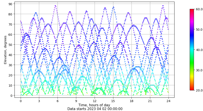
Time-elevation plot for station TALR. Signal to Noise S1C Data file TALR00ESP_R_2023092.xtr
