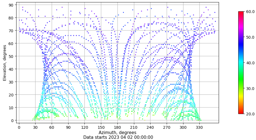
Azimuth-elevation plot for station TALR. Signal to Noise S1C Data file TALR00ESP_R_2023092.xtr
