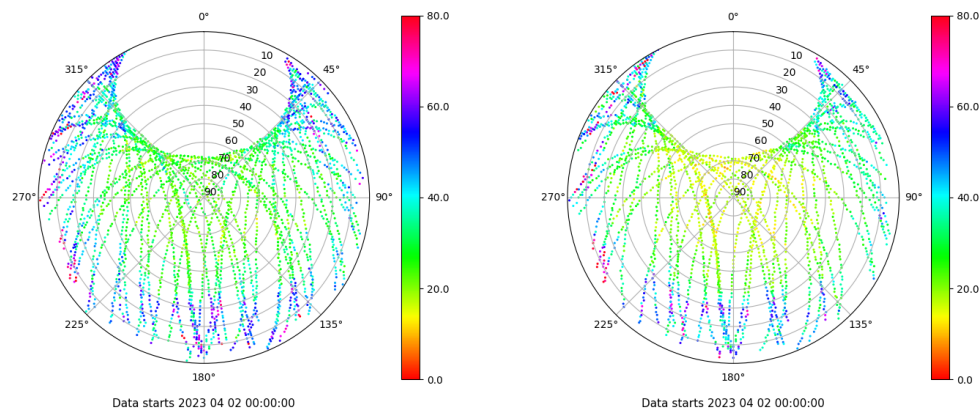
Skyplot for station TALR. Parameter M1C Data file TALR00ESP_R_2023092.xtr Skyplot for station TALR. Parameter M2X Data file TALR00ESP_R_2023092.xtr
