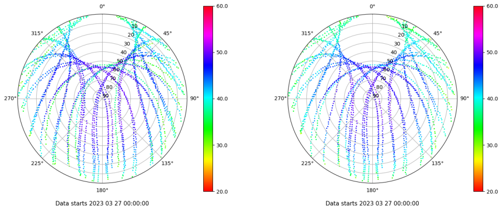
Skyplot for station TALR. Signal to Noise S1C Data file TALR00ESP_R_2023086.xtr Skyplot for station TALR. Signal to Noise S2C Data file TALR00ESP_R_2023086.xtr
