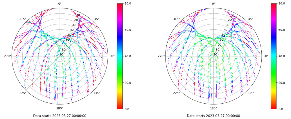
Skyplot for station TALR. Parameter M1C Data file TALR00ESP_R_2023086.xtr Skyplot for station TALR. Parameter M2C Data file TALR00ESP_R_2023086.xtr
