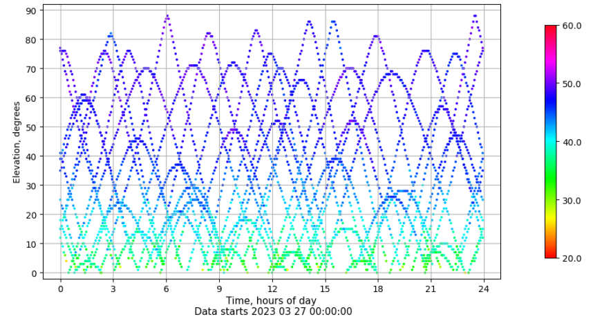
Time-elevation plot for station TALR. Signal to Noise S1C Data file TALR00ESP_R_2023086.xtr
