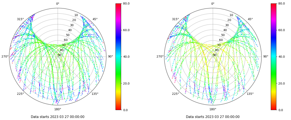
Skyplot for station TALR. Parameter M1C Data file TALR00ESP_R_2023086.xtr Skyplot for station TALR. Parameter M2X Data file TALR00ESP_R_2023086.xtr
