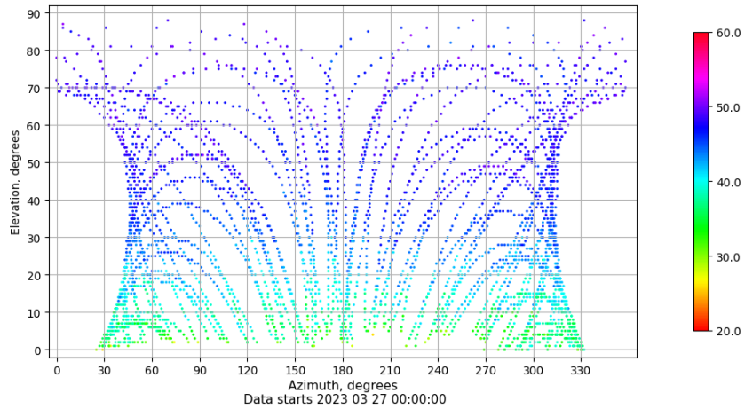
Azimuth-elevation plot for station TALR. Signal to Noise S1C Data file TALR00ESP_R_2023086.xtr
