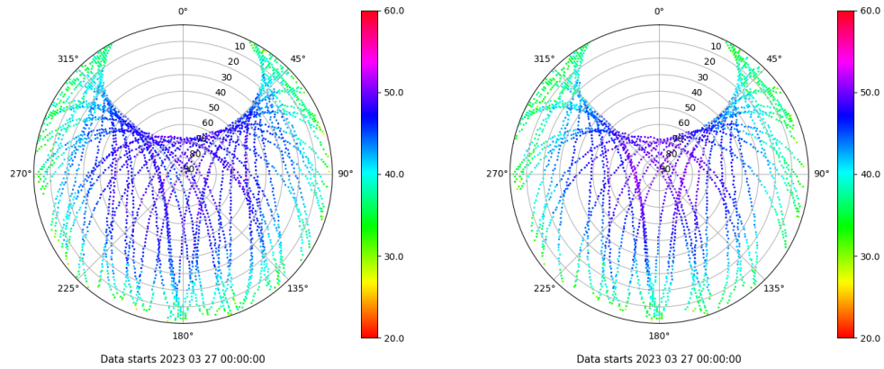
Skyplot for station TALR. Signal to Noise S1C Data file TALR00ESP_R_2023086.xtr Skyplot for station TALR. Signal to Noise S2X Data file TALR00ESP_R_2023086.xtr
