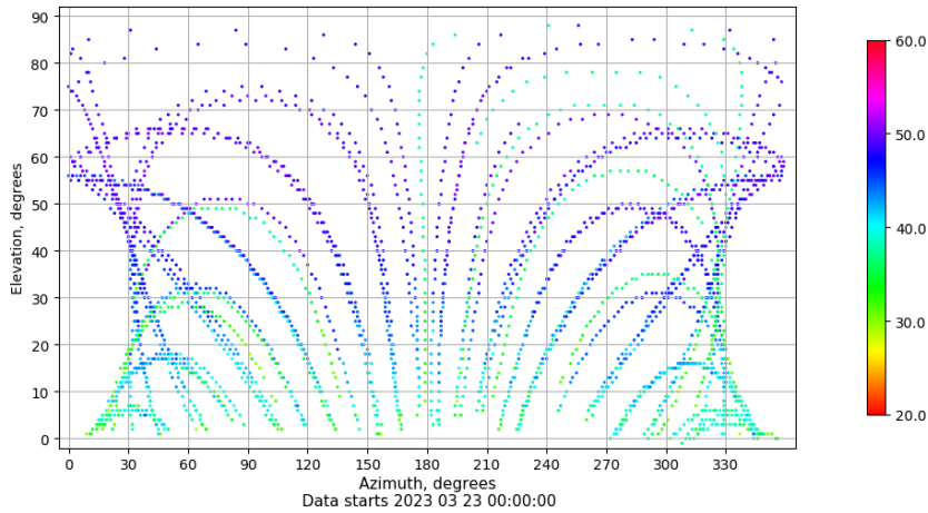
Azimuth-elevation plot for station TALR. Signal to Noise S1C Data file TALR00ESP_R_2023082.xtr
