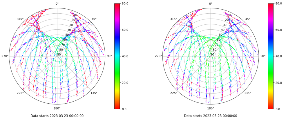
Skyplot for station TALR. Parameter M1C Data file TALR00ESP_R_2023082.xtr Skyplot for station TALR. Parameter M2C Data file TALR00ESP_R_2023082.xtr
