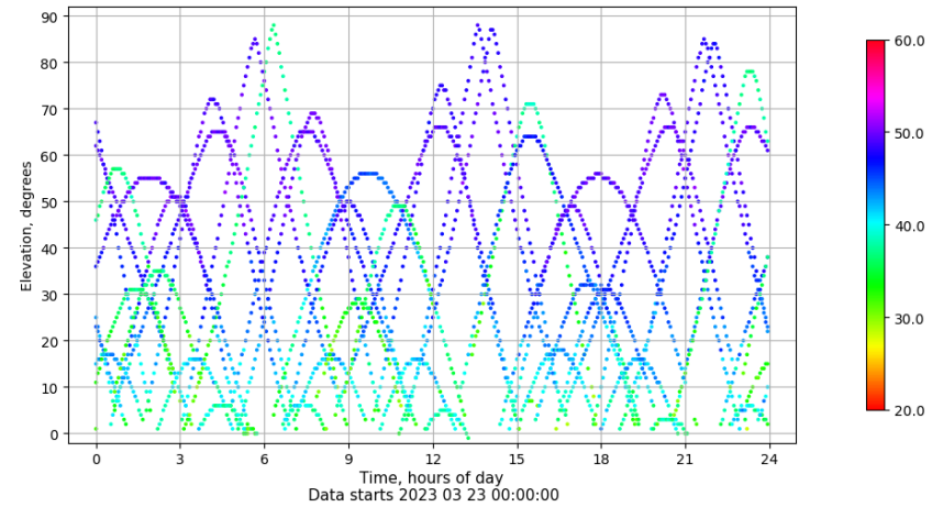
Time-elevation plot for station TALR. Signal to Noise S1C Data file TALR00ESP_R_2023082.xtr
