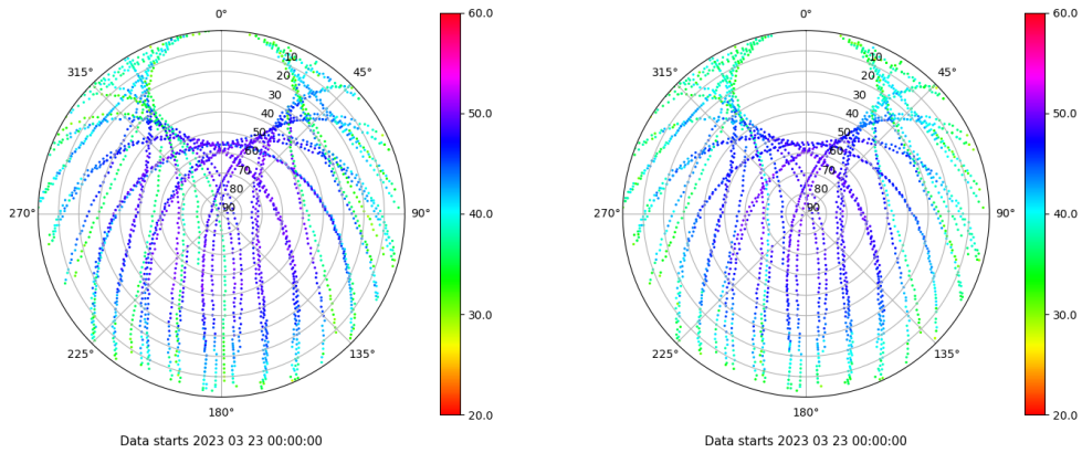
Skyplot for station TALR. Signal to Noise S1C Data file TALR00ESP_R_2023082.xtr Skyplot for station TALR. Signal to Noise S2C Data file TALR00ESP_R_2023082.xtr
