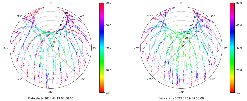
Skyplot for station TALR. Parameter M1C Data file TALR00ESP_R_2023078.xtr Skyplot for station TALR. Parameter M2C Data file TALR00ESP_R_2023078.xtr
