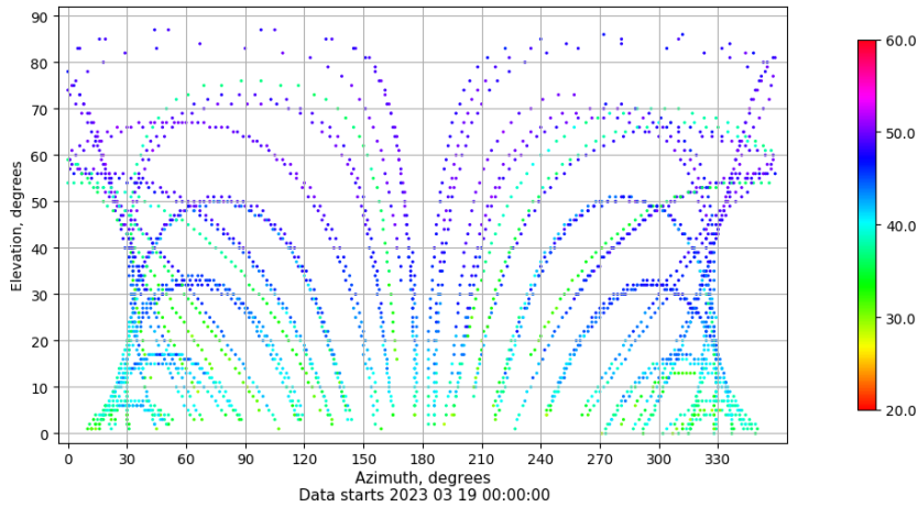
Azimuth-elevation plot for station TALR. Signal to Noise S1C Data file TALR00ESP_R_2023078.xtr
