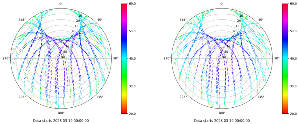
Skyplot for station TALR. Signal to Noise S1C Data file TALR00ESP_R_2023078.xtr Skyplot for station TALR. Signal to Noise S2C Data file TALR00ESP_R_2023078.xtr
