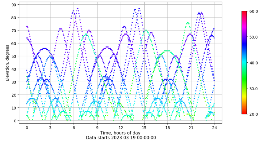
Time-elevation plot for station TALR. Signal to Noise S1C Data file TALR00ESP_R_2023078.xtr
