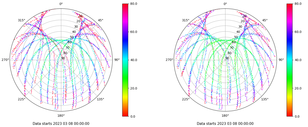
Skyplot for station TALR. Parameter M1C Data file TALR00ESP_R_2023067.xtr Skyplot for station TALR. Parameter M2C Data file TALR00ESP_R_2023067.xtr
