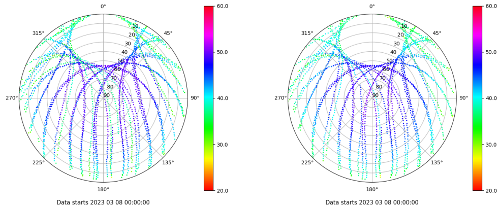
Skyplot for station TALR. Signal to Noise S1C Data file TALR00ESP_R_2023067.xtr Skyplot for station TALR. Signal to Noise S2C Data file TALR00ESP_R_2023067.xtr
