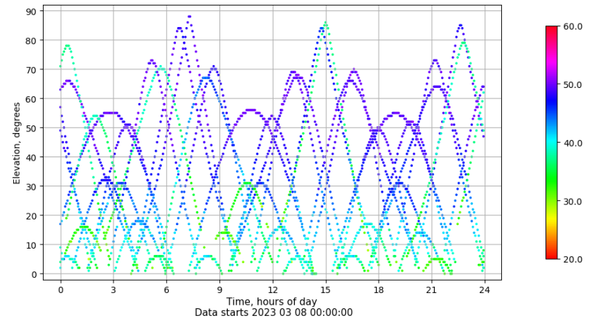
Time-elevation plot for station TALR. Signal to Noise S1C Data file TALR00ESP_R_2023067.xtr
