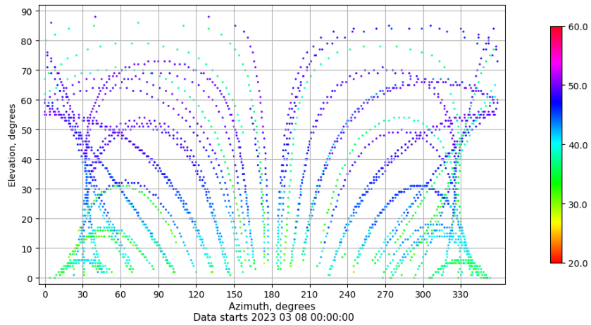
Azimuth-elevation plot for station TALR. Signal to Noise S1C Data file TALR00ESP_R_2023067.xtr
