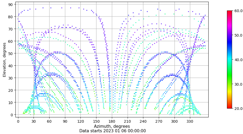
Azimuth-elevation plot for station TALR. Signal to Noise S1C Data file TALR00ESP_R_2023006.xtr
