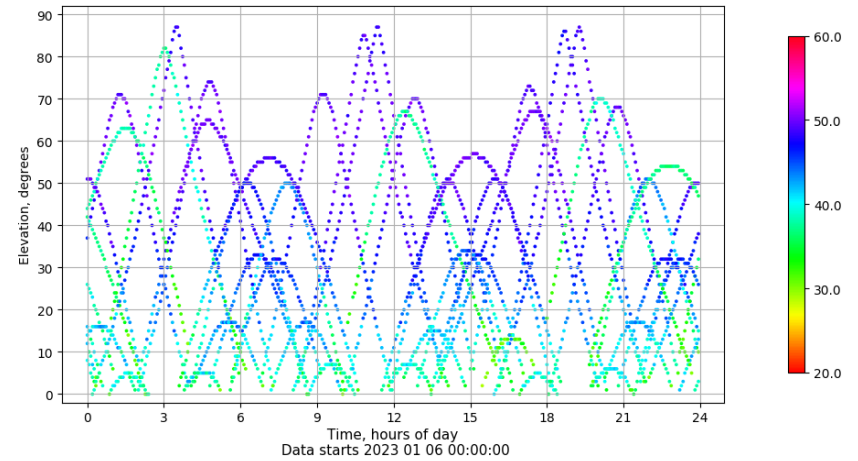
Time-elevation plot for station TALR. Signal to Noise S1C Data file TALR00ESP_R_2023006.xtr
