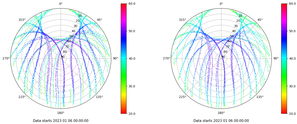
Skyplot for station TALR. Signal to Noise S1C Data file TALR00ESP_R_2023006.xtr Skyplot for station TALR. Signal to Noise S2C Data file TALR00ESP_R_2023006.xtr
