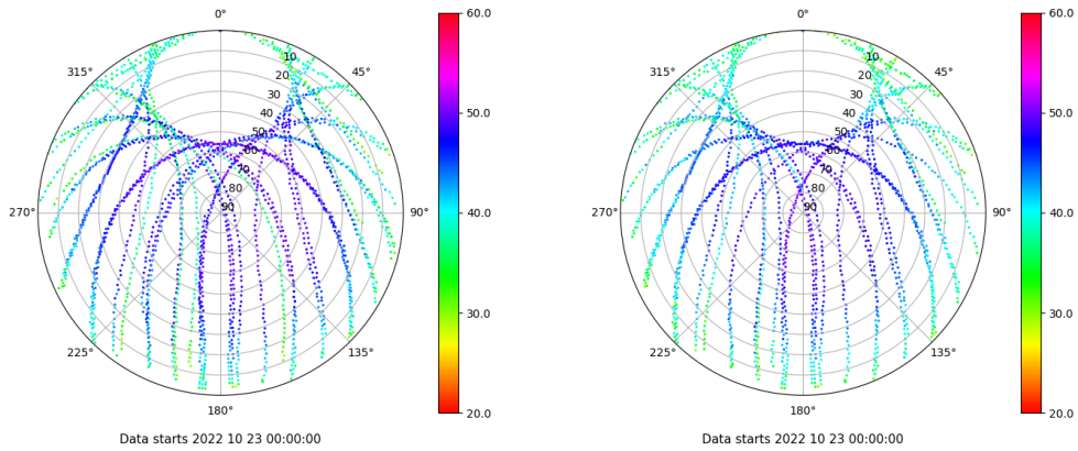
Skyplot for station TALR. Signal to Noise S1C Data file TALR00ESP_R_2022296.xtr Skyplot for station TALR. Signal to Noise S2C Data file TALR00ESP_R_2022296.xtr
