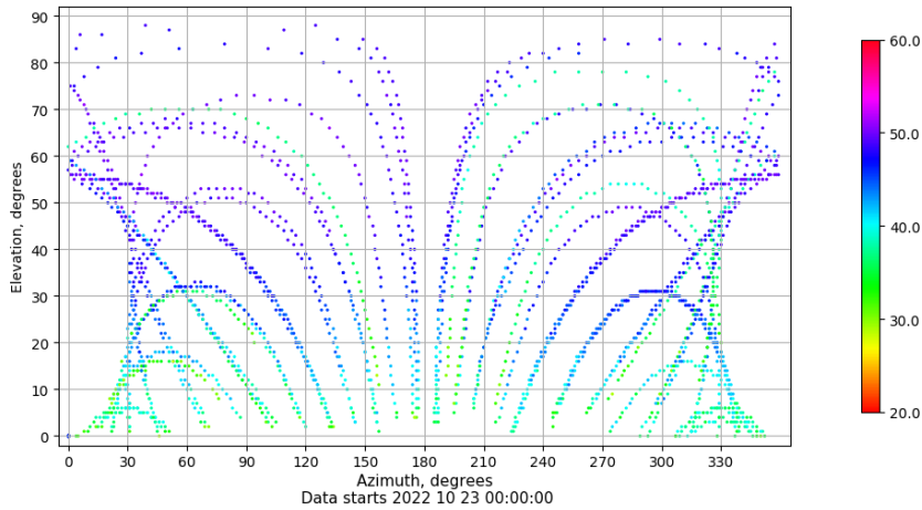
Azimuth-elevation plot for station TALR. Signal to Noise S1C Data file TALR00ESP_R_2022296.xtr
