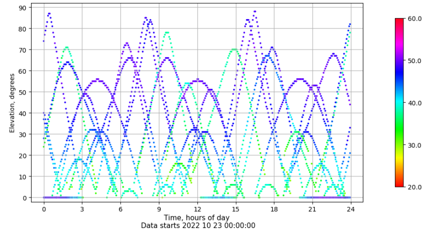
Time-elevation plot for station TALR. Signal to Noise S1C Data file TALR00ESP_R_2022296.xtr
