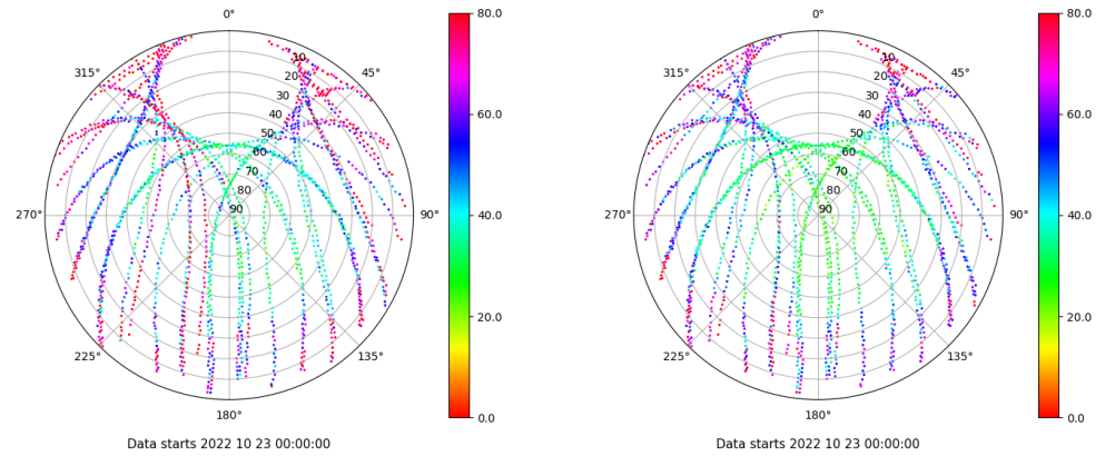
Skyplot for station TALR. Parameter M1C Data file TALR00ESP_R_2022296.xtr Skyplot for station TALR. Parameter M2C Data file TALR00ESP_R_2022296.xtr
