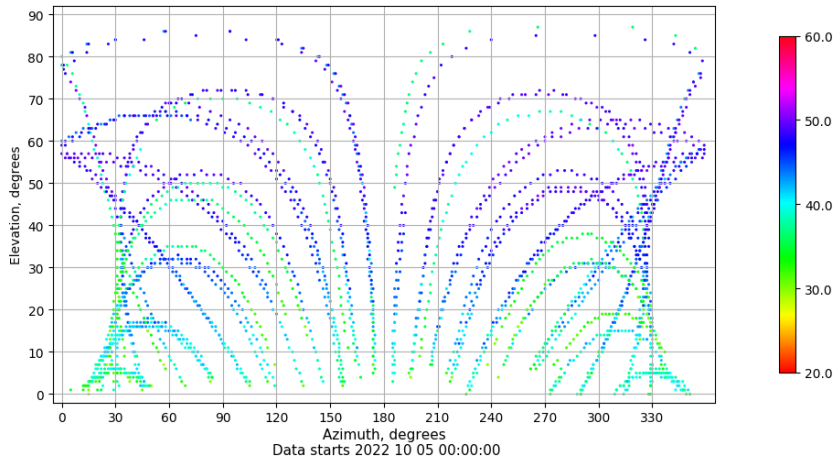
Azimuth-elevation plot for station TALR. Signal to Noise S1C Data file TALR00ESP_R_2022278.xtr
