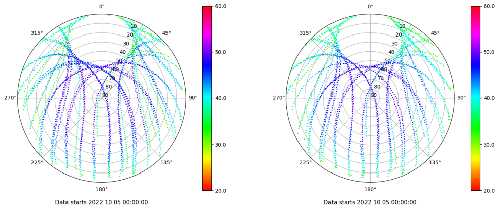
Skyplot for station TALR. Signal to Noise S1C Data file TALR00ESP_R_2022278.xtr Skyplot for station TALR. Signal to Noise S2C Data file TALR00ESP_R_2022278.xtr
