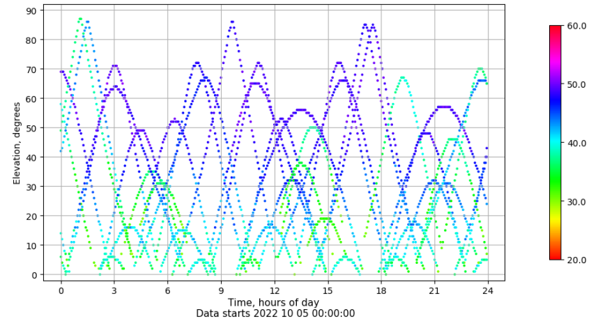
Time-elevation plot for station TALR. Signal to Noise S1C Data file TALR00ESP_R_2022278.xtr
