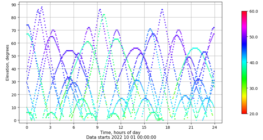
Time-elevation plot for station TALR. Signal to Noise S1C Data file TALR00ESP_R_2022274.xtr
