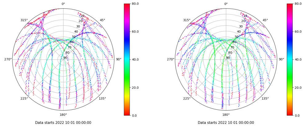
Skyplot for station TALR. Parameter M1C Data file TALR00ESP_R_2022274.xtr Skyplot for station TALR. Parameter M2C Data file TALR00ESP_R_2022274.xtr
