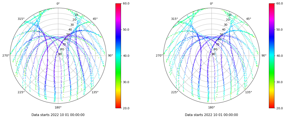
Skyplot for station TALR. Signal to Noise S1C Data file TALR00ESP_R_2022274.xtr Skyplot for station TALR. Signal to Noise S2C Data file TALR00ESP_R_2022274.xtr
