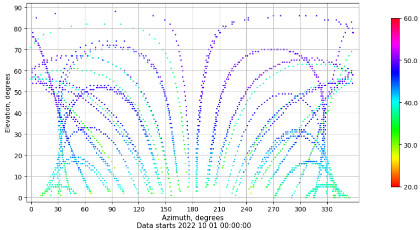
Azimuth-elevation plot for station TALR. Signal to Noise S1C Data file TALR00ESP_R_2022274.xtr
