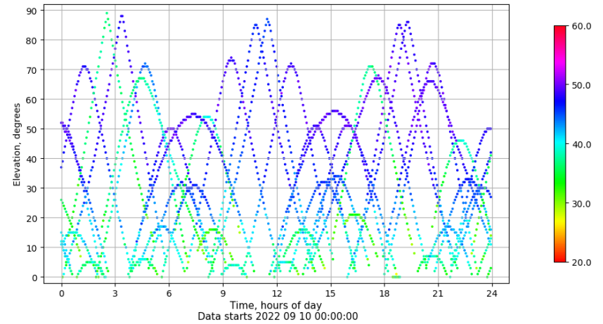
Time-elevation plot for station TALR. Signal to Noise S1C Data file TALR00ESP_R_2022253.xtr
