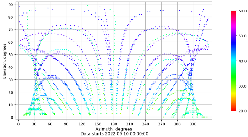
Azimuth-elevation plot for station TALR. Signal to Noise S1C Data file TALR00ESP_R_2022253.xtr
