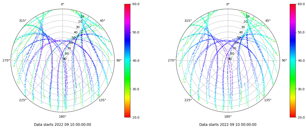
Skyplot for station TALR. Signal to Noise S1C Data file TALR00ESP_R_2022253.xtr Skyplot for station TALR. Signal to Noise S2C Data file TALR00ESP_R_2022253.xtr
