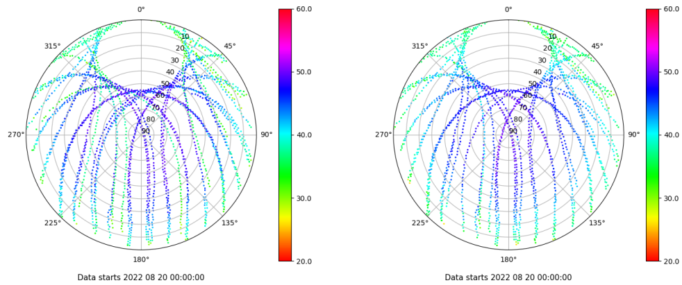
Skyplot for station TALR. Signal to Noise S1C Data file TALR00ESP_R_2022232.xtr Skyplot for station TALR. Signal to Noise S2C Data file TALR00ESP_R_2022232.xtr
