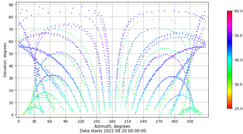
Azimuth-elevation plot for station TALR. Signal to Noise S1C Data file TALR00ESP_R_2022232.xtr
