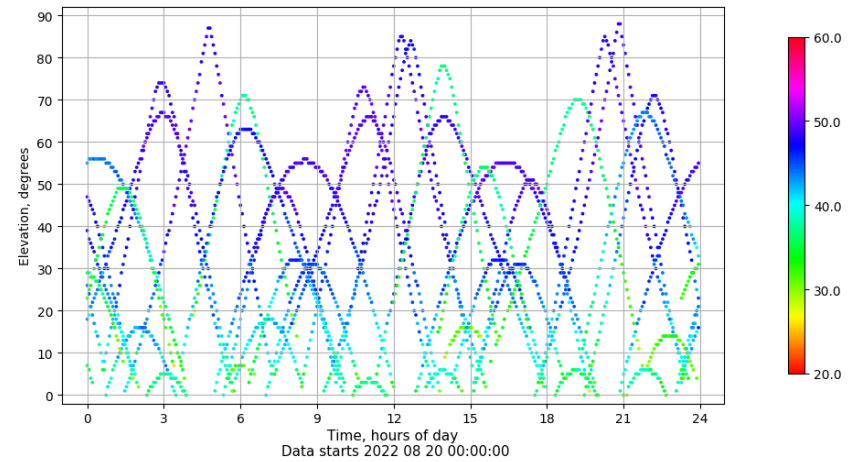
Time-elevation plot for station TALR. Signal to Noise S1C Data file TALR00ESP_R_2022232.xtr
