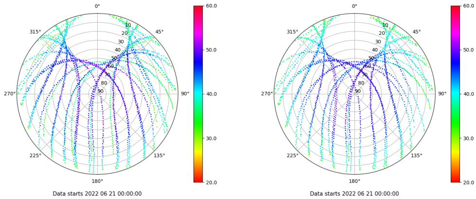
Skyplot for station TALR. Signal to Noise S1C Data file TALR00ESP_R_2022172.xtr Skyplot for station TALR. Signal to Noise S2C Data file TALR00ESP_R_2022172.xtr
