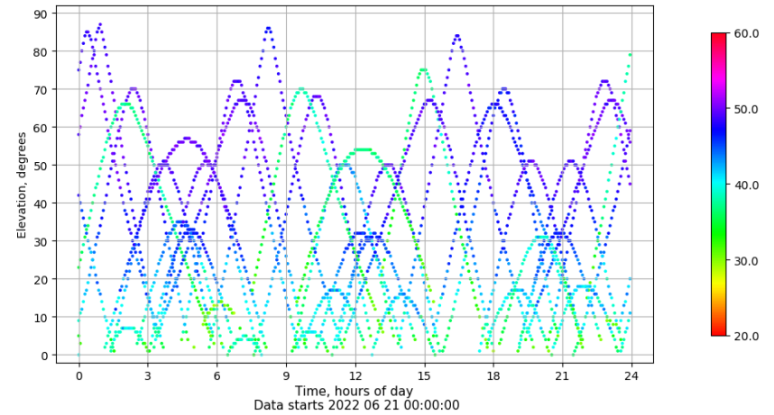
Time-elevation plot for station TALR. Signal to Noise S1C Data file TALR00ESP_R_2022172.xtr
