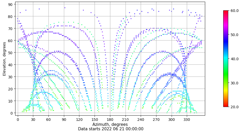
Azimuth-elevation plot for station TALR. Signal to Noise S1C Data file TALR00ESP_R_2022172.xtr
