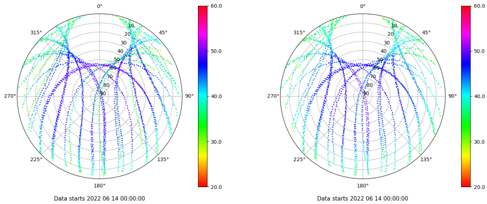
Skyplot for station TALR. Signal to Noise S1C Data file TALR00ESP_R_2022165.xtr Skyplot for station TALR. Signal to Noise S2C Data file TALR00ESP_R_2022165.xtr
