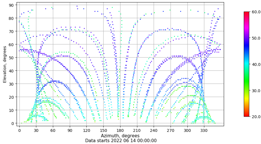
Azimuth-elevation plot for station TALR. Signal to Noise S1C Data file TALR00ESP_R_2022165.xtr
