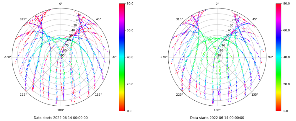
Skyplot for station TALR. Parameter M1C Data file TALR00ESP_R_2022165.xtr Skyplot for station TALR. Parameter M2C Data file TALR00ESP_R_2022165.xtr
