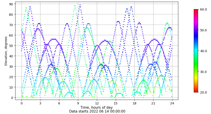
Time-elevation plot for station TALR. Signal to Noise S1C Data file TALR00ESP_R_2022165.xtr
