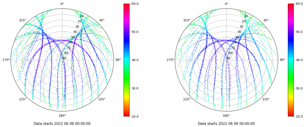
Skyplot for station TALR. Signal to Noise S1C Data file TALR00ESP_R_2022157.xtr Skyplot for station TALR. Signal to Noise S2C Data file TALR00ESP_R_2022157.xtr
