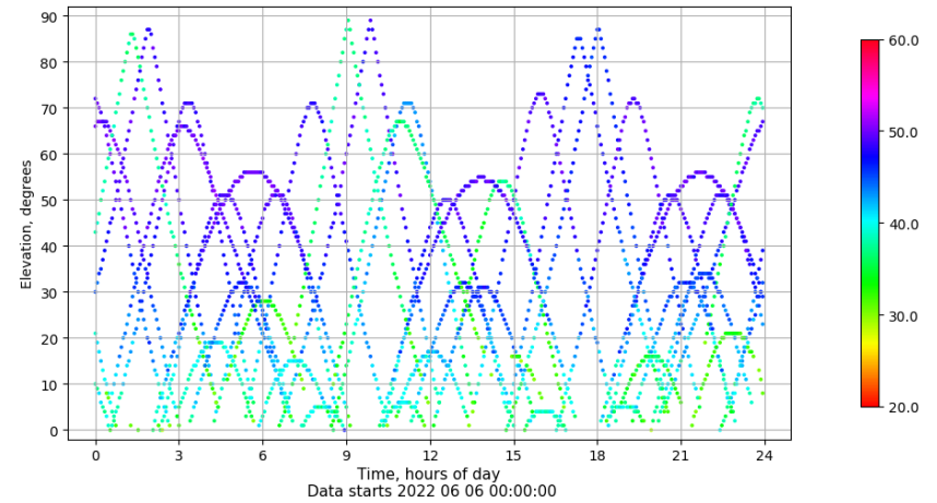
Time-elevation plot for station TALR. Signal to Noise S1C Data file TALR00ESP_R_2022157.xtr
