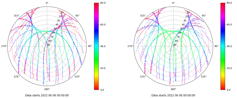
Skyplot for station TALR. Parameter M1C Data file TALR00ESP_R_2022157.xtr Skyplot for station TALR. Parameter M2C Data file TALR00ESP_R_2022157.xtr
