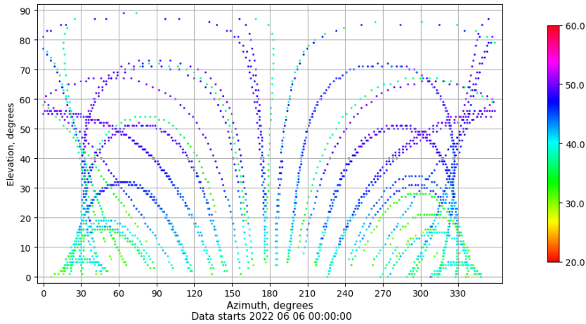
Azimuth-elevation plot for station TALR. Signal to Noise S1C Data file TALR00ESP_R_2022157.xtr
