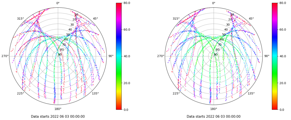
Skyplot for station TALR. Parameter M1C Data file TALR00ESP_R_2022154.xtr Skyplot for station TALR. Parameter M2C Data file TALR00ESP_R_2022154.xtr
