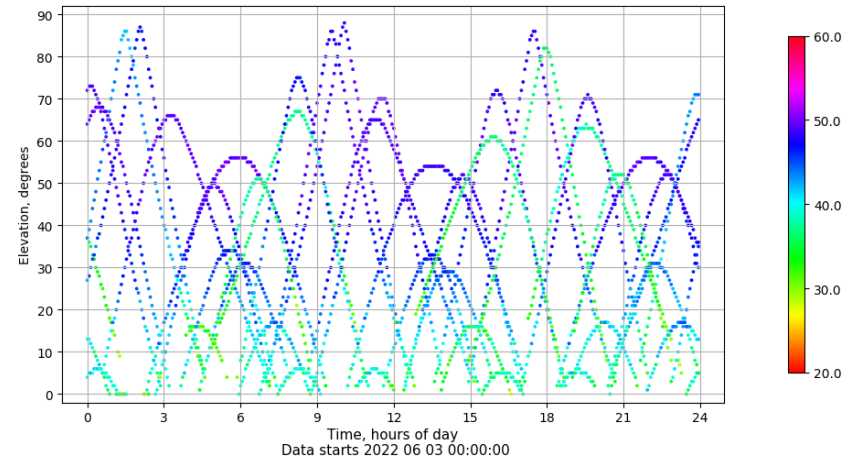
Time-elevation plot for station TALR. Signal to Noise S1C Data file TALR00ESP_R_2022154.xtr
