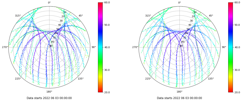
Skyplot for station TALR. Signal to Noise S1C Data file TALR00ESP_R_2022154.xtr Skyplot for station TALR. Signal to Noise S2C Data file TALR00ESP_R_2022154.xtr
