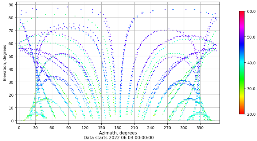
Azimuth-elevation plot for station TALR. Signal to Noise S1C Data file TALR00ESP_R_2022154.xtr
