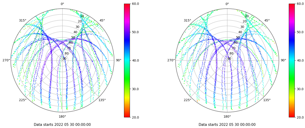
Skyplot for station TALR. Signal to Noise S1C Data file TALR00ESP_R_2022150.xtr Skyplot for station TALR. Signal to Noise S2C Data file TALR00ESP_R_2022150.xtr
