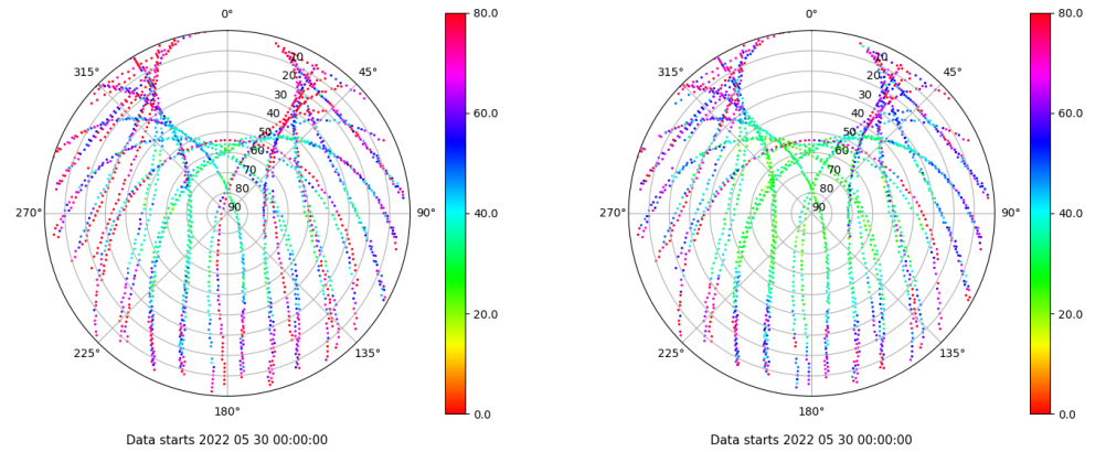
Skyplot for station TALR. Parameter M1C Data file TALR00ESP_R_2022150.xtr Skyplot for station TALR. Parameter M2C Data file TALR00ESP_R_2022150.xtr
