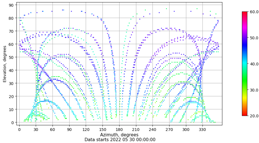
Azimuth-elevation plot for station TALR. Signal to Noise S1C Data file TALR00ESP_R_2022150.xtr
