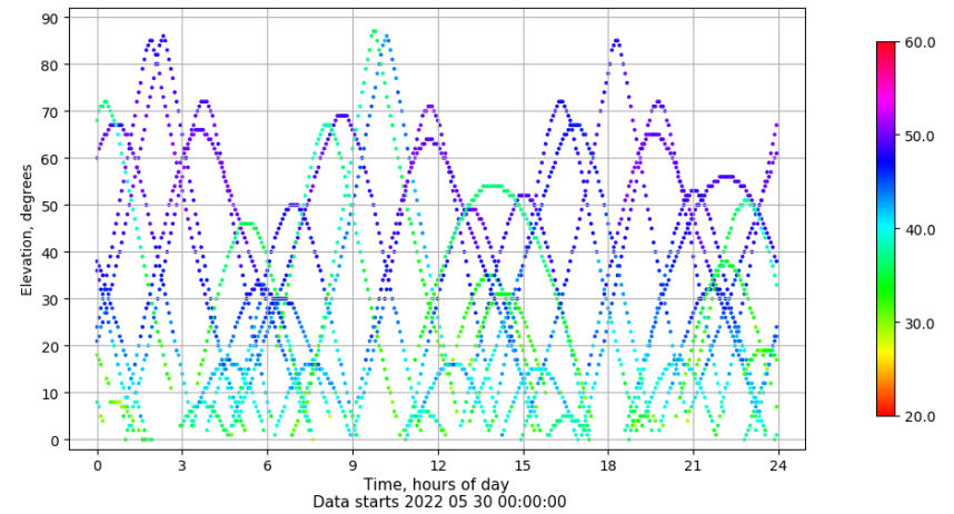
Time-elevation plot for station TALR. Signal to Noise S1C Data file TALR00ESP_R_2022150.xtr
