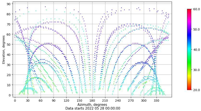
Azimuth-elevation plot for station TALR. Signal to Noise S1C Data file TALR00ESP_R_2022148.xtr
