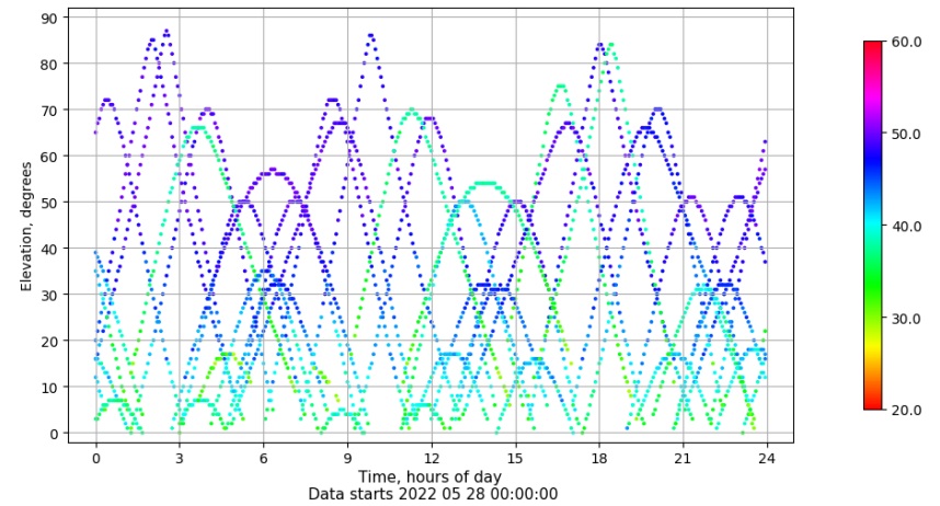
Time-elevation plot for station TALR. Signal to Noise S1C Data file TALR00ESP_R_2022148.xtr
