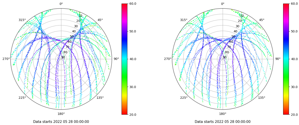
Skyplot for station TALR. Signal to Noise S1C Data file TALR00ESP_R_2022148.xtr Skyplot for station TALR. Signal to Noise S2C Data file TALR00ESP_R_2022148.xtr
