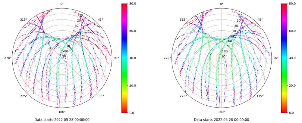
Skyplot for station TALR. Parameter M1C Data file TALR00ESP_R_2022148.xtr Skyplot for station TALR. Parameter M2C Data file TALR00ESP_R_2022148.xtr
