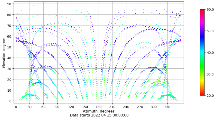
Azimuth-elevation plot for station TALR. Signal to Noise S1C Data file TALR00ESP_R_2022105.xtr
