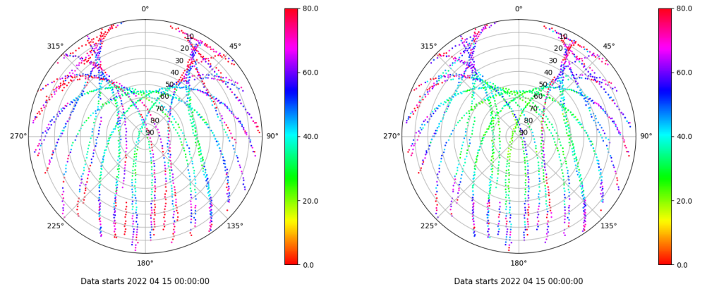
Skyplot for station TALR. Parameter M1C Data file TALR00ESP_R_2022105.xtr Skyplot for station TALR. Parameter M2C Data file TALR00ESP_R_2022105.xtr
