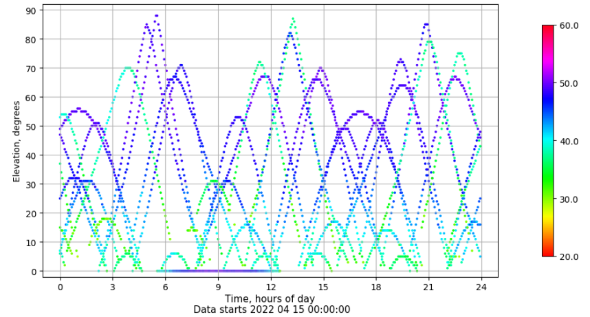
Time-elevation plot for station TALR. Signal to Noise S1C Data file TALR00ESP_R_2022105.xtr
