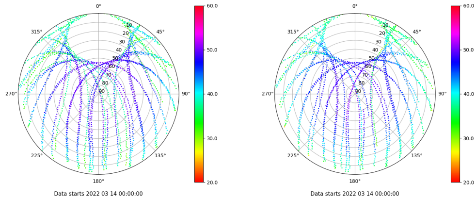
Skyplot for station TALR. Signal to Noise S1C Data file TALR00ESP_R_2022073.xtr Skyplot for station TALR. Signal to Noise S2C Data file TALR00ESP_R_2022073.xtr
