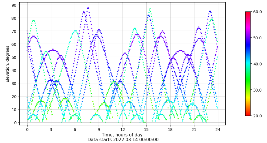
Time-elevation plot for station TALR. Signal to Noise S1C Data file TALR00ESP_R_2022073.xtr
