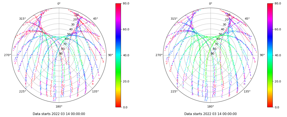
Skyplot for station TALR. Parameter M1C Data file TALR00ESP_R_2022073.xtr Skyplot for station TALR. Parameter M2C Data file TALR00ESP_R_2022073.xtr
