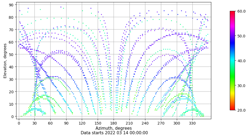
Azimuth-elevation plot for station TALR. Signal to Noise S1C Data file TALR00ESP_R_2022073.xtr
