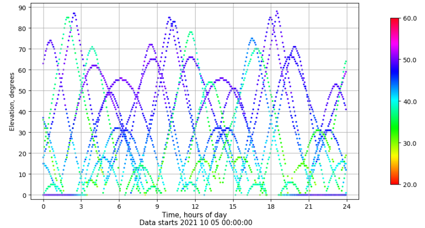
Time-elevation plot for station TALR. Signal to Noise S1C Data file TALR00ESP_R_2021278.xtr
