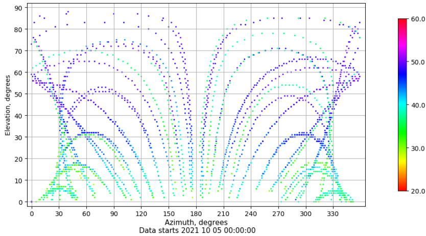
Azimuth-elevation plot for station TALR. Signal to Noise S1C Data file TALR00ESP_R_2021278.xtr
