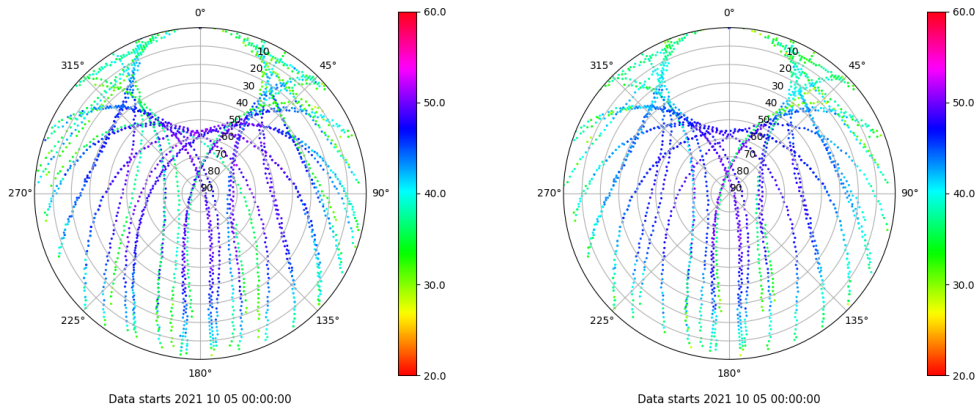
Skyplot for station TALR. Signal to Noise S1C Data file TALR00ESP_R_2021278.xtr Skyplot for station TALR. Signal to Noise S2C Data file TALR00ESP_R_2021278.xtr
