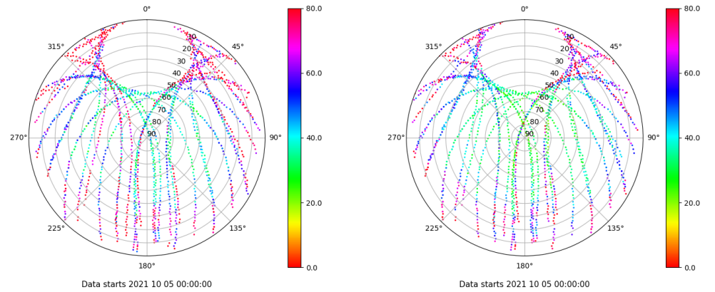
Skyplot for station TALR. Parameter M1C Data file TALR00ESP_R_2021278.xtr Skyplot for station TALR. Parameter M2C Data file TALR00ESP_R_2021278.xtr
