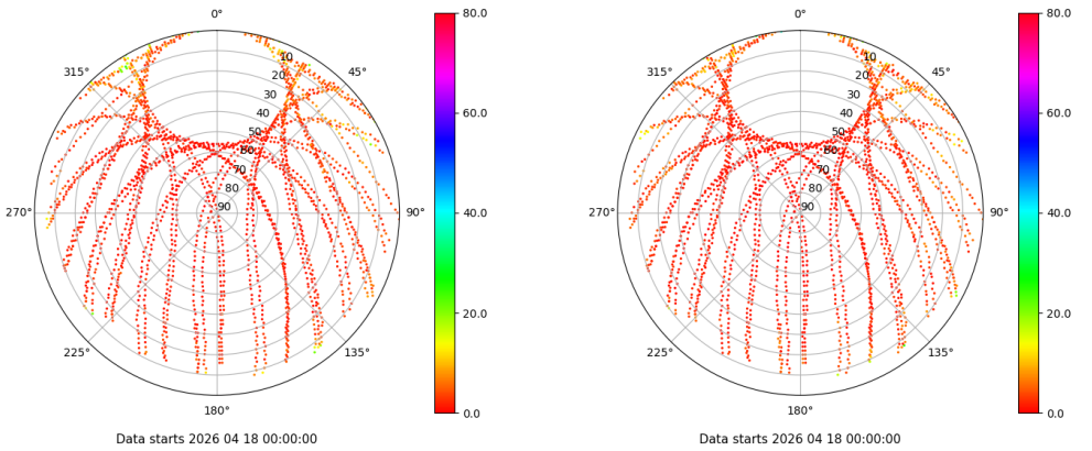
Skyplot for station SPAB. Parameter M1C Data file SPAB00ESP_R_2026108.xtr Skyplot for station SPAB. Parameter M2P Data file SPAB00ESP_R_2026108.xtr
