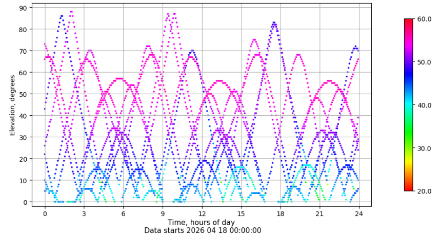
Time-elevation plot for station SPAB. Signal to Noise S1C Data file SPAB00ESP_R_2026108.xtr
