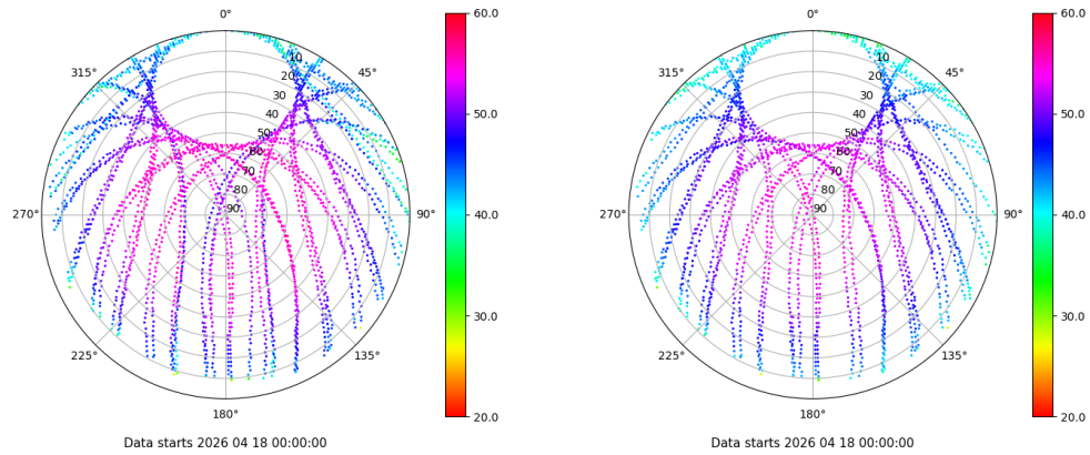
Skyplot for station SPAB. Signal to Noise S1C Data file SPAB00ESP_R_2026108.xtr Skyplot for station SPAB. Signal to Noise S2P Data file SPAB00ESP_R_2026108.xtr
