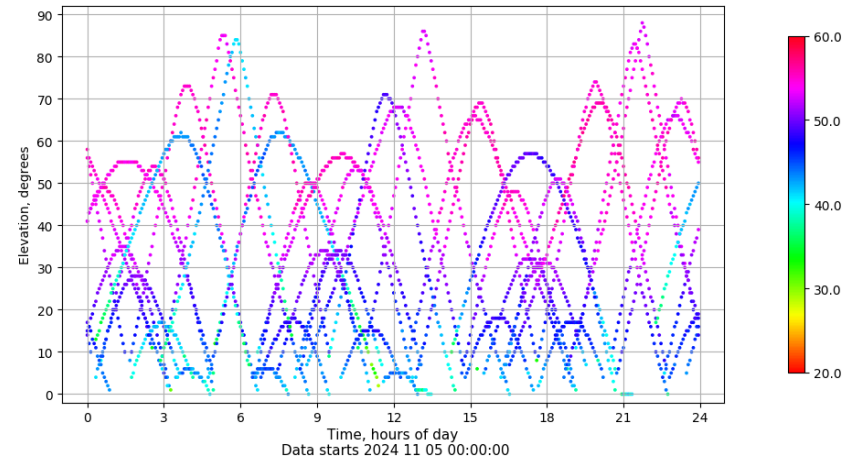
Time-elevation plot for station SPAB. Signal to Noise S1C Data file SPAB00ESP_R_2024310.xtr
