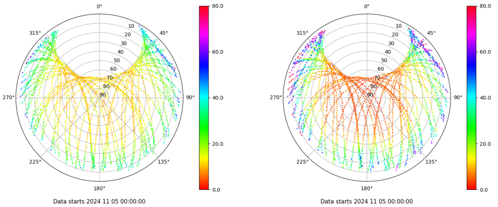
Skyplot for station SPAB. Parameter M1C Data file SPAB00ESP_R_2024310.xtr Skyplot for station SPAB. Parameter M2W Data file SPAB00ESP_R_2024310.xtr
