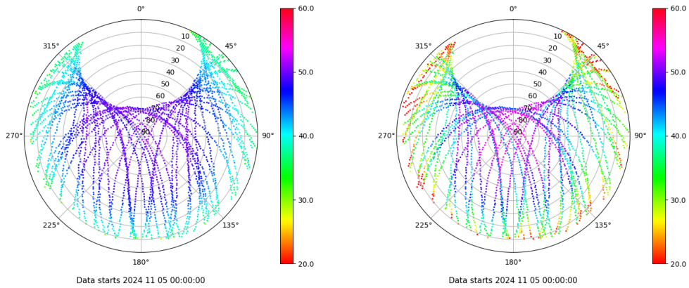
Skyplot for station SPAB. Signal to Noise S1C Data file SPAB00ESP_R_2024310.xtr Skyplot for station SPAB. Signal to Noise S2W Data file SPAB00ESP_R_2024310.xtr
