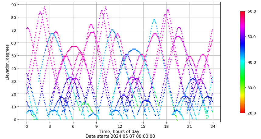
Time-elevation plot for station SPAB. Signal to Noise S1C Data file SPAB00ESP_R_2024128.xtr
