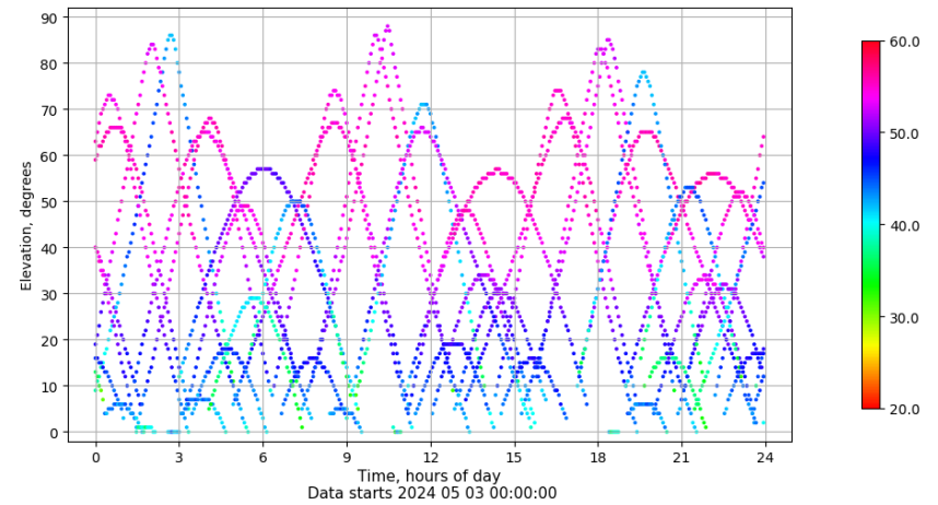
Time-elevation plot for station SPAB. Signal to Noise S1C Data file SPAB00ESP_R_2024124.xtr
