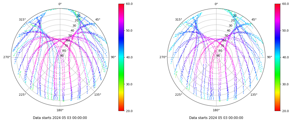
Skyplot for station SPAB. Signal to Noise S1C Data file SPAB00ESP_R_2024124.xtr Skyplot for station SPAB. Signal to Noise S2P Data file SPAB00ESP_R_2024124.xtr
