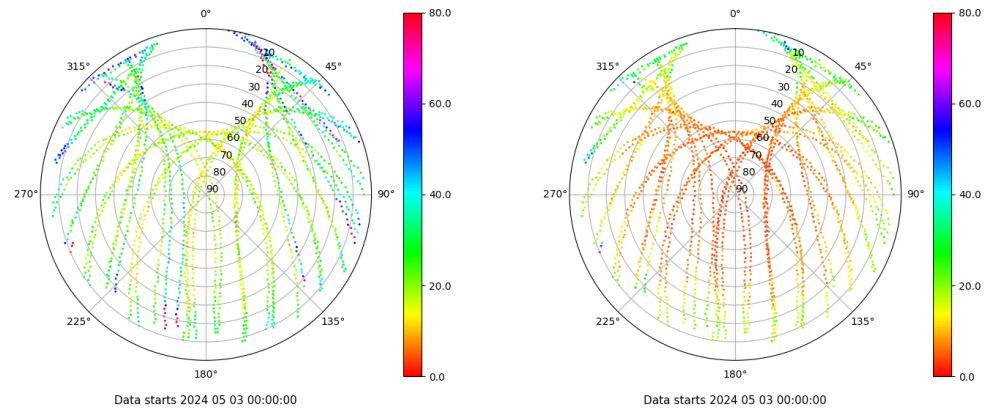
Skyplot for station SPAB. Parameter M1C Data file SPAB00ESP_R_2024124.xtr Skyplot for station SPAB. Parameter M2P Data file SPAB00ESP_R_2024124.xtr
