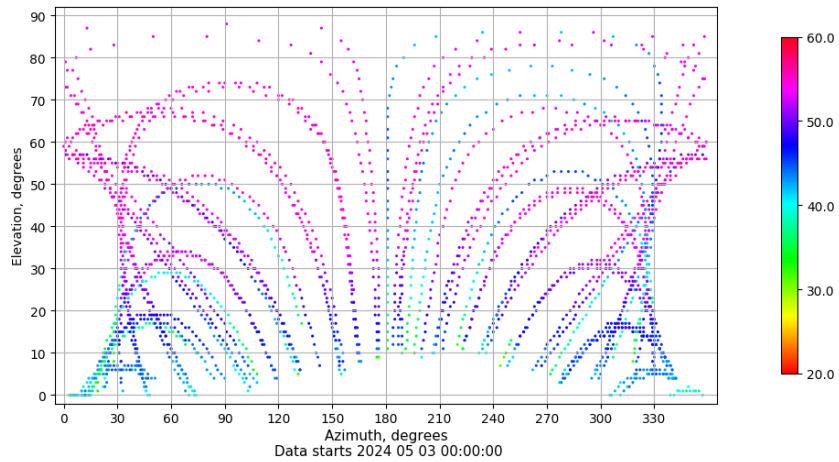
Azimuth-elevation plot for station SPAB. Signal to Noise S1C Data file SPAB00ESP_R_2024124.xtr
