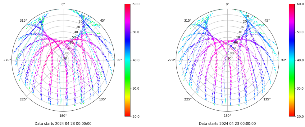
Skyplot for station SPAB. Signal to Noise S1C Data file SPAB00ESP_R_2024114.xtr Skyplot for station SPAB. Signal to Noise S2P Data file SPAB00ESP_R_2024114.xtr
