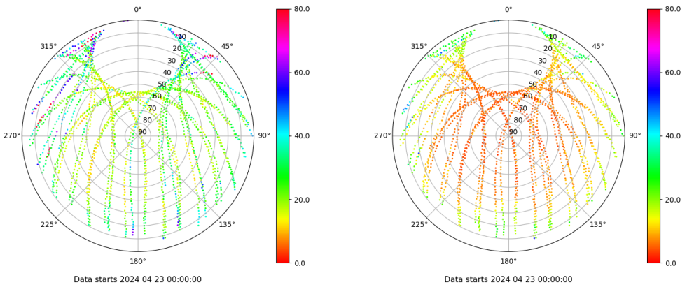
Skyplot for station SPAB. Parameter M1C Data file SPAB00ESP_R_2024114.xtr Skyplot for station SPAB. Parameter M2P Data file SPAB00ESP_R_2024114.xtr
