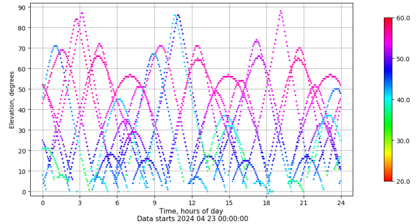
Time-elevation plot for station SPAB. Signal to Noise S1C Data file SPAB00ESP_R_2024114.xtr
