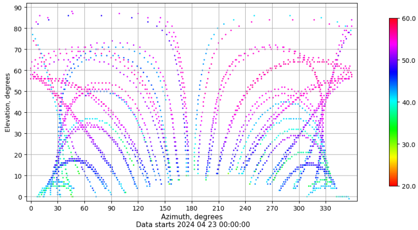
Azimuth-elevation plot for station SPAB. Signal to Noise S1C Data file SPAB00ESP_R_2024114.xtr
