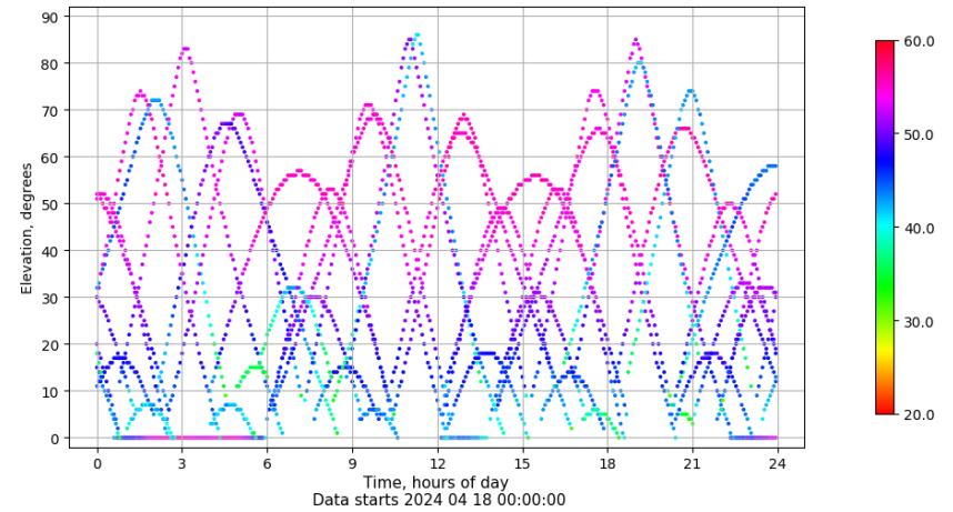
Time-elevation plot for station SPAB. Signal to Noise S1C Data file SPAB00ESP_R_2024109.xtr
