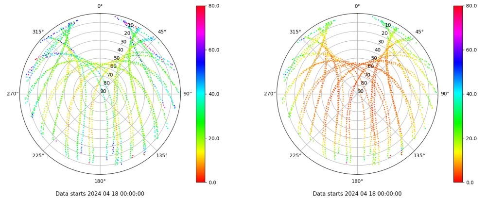
Skyplot for station SPAB. Parameter M1C Data file SPAB00ESP_R_2024109.xtr Skyplot for station SPAB. Parameter M2P Data file SPAB00ESP_R_2024109.xtr
