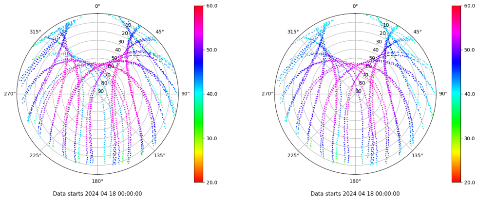
Skyplot for station SPAB. Signal to Noise S1C Data file SPAB00ESP_R_2024109.xtr Skyplot for station SPAB. Signal to Noise S2P Data file SPAB00ESP_R_2024109.xtr
