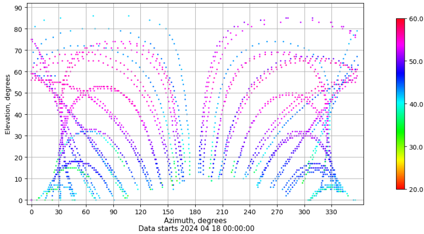
Azimuth-elevation plot for station SPAB. Signal to Noise S1C Data file SPAB00ESP_R_2024109.xtr
