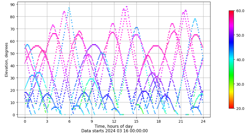
Time-elevation plot for station SPAB. Signal to Noise S1C Data file SPAB00ESP_R_2024076.xtr
