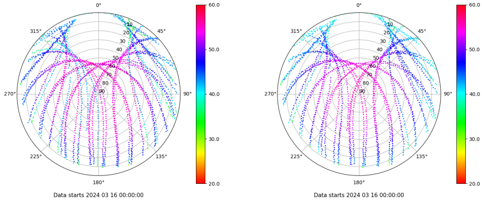
Skyplot for station SPAB. Signal to Noise S1C Data file SPAB00ESP_R_2024076.xtr Skyplot for station SPAB. Signal to Noise S2P Data file SPAB00ESP_R_2024076.xtr
