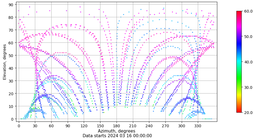
Azimuth-elevation plot for station SPAB. Signal to Noise S1C Data file SPAB00ESP_R_2024076.xtr
