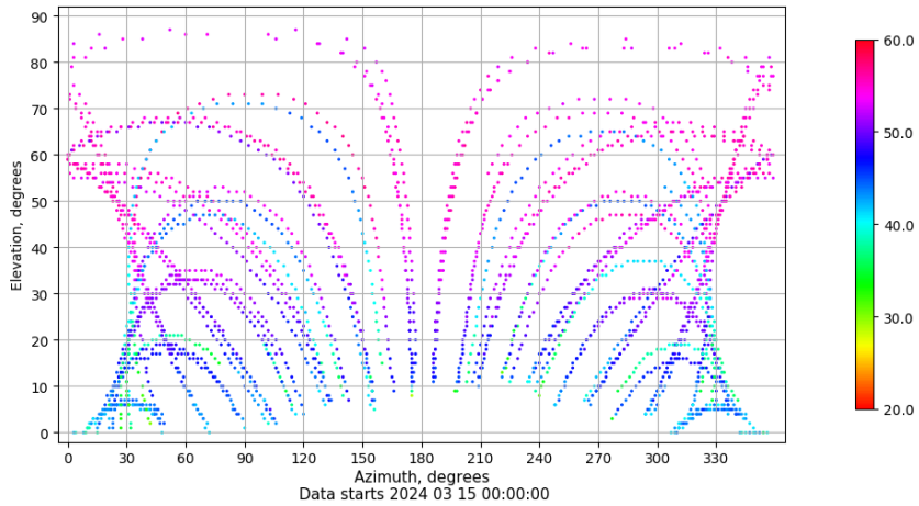
Azimuth-elevation plot for station SPAB. Signal to Noise S1C Data file SPAB00ESP_R_2024075.xtr
