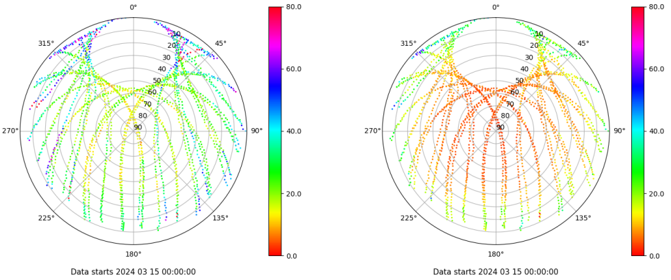
Skyplot for station SPAB. Parameter M1C Data file SPAB00ESP_R_2024075.xtr Skyplot for station SPAB. Parameter M2P Data file SPAB00ESP_R_2024075.xtr
