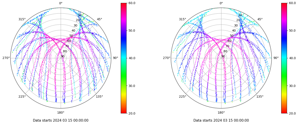
Skyplot for station SPAB. Signal to Noise S1C Data file SPAB00ESP_R_2024075.xtr Skyplot for station SPAB. Signal to Noise S2P Data file SPAB00ESP_R_2024075.xtr
