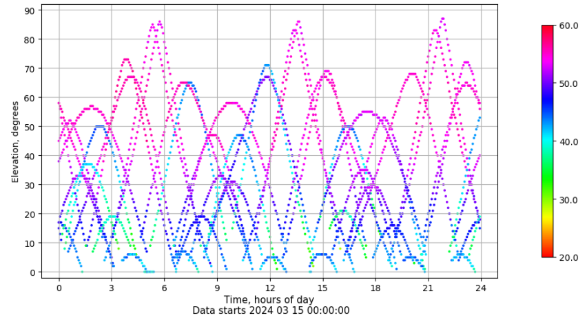
Time-elevation plot for station SPAB. Signal to Noise S1C Data file SPAB00ESP_R_2024075.xtr
