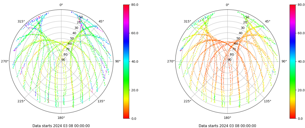
Skyplot for station SPAB. Parameter M1C Data file SPAB00ESP_R_2024068.xtr Skyplot for station SPAB. Parameter M2P Data file SPAB00ESP_R_2024068.xtr
