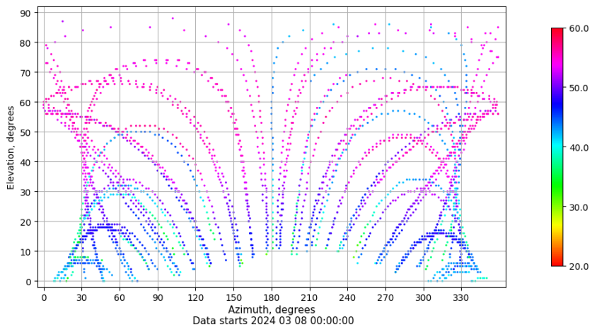
Azimuth-elevation plot for station SPAB. Signal to Noise S1C Data file SPAB00ESP_R_2024068.xtr
