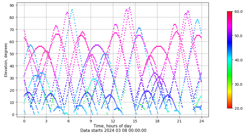
Time-elevation plot for station SPAB. Signal to Noise S1C Data file SPAB00ESP_R_2024068.xtr
