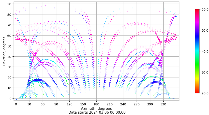
Azimuth-elevation plot for station SPAB. Signal to Noise S1C Data file SPAB00ESP_R_2024066.xtr
