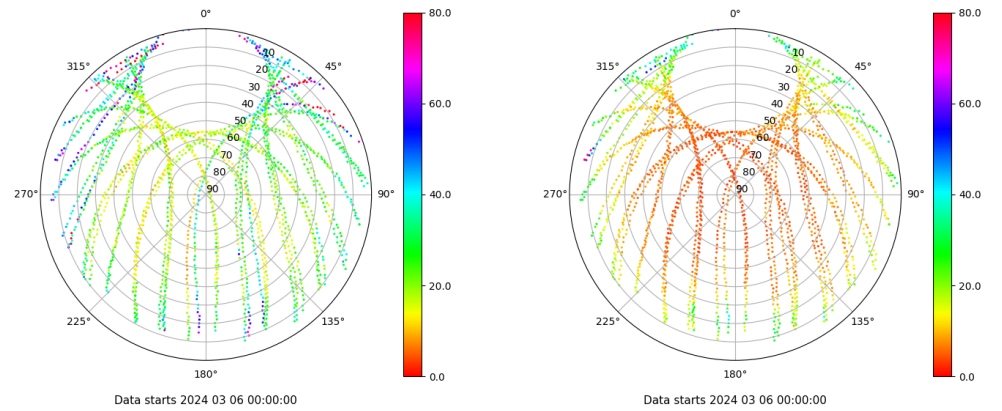
Skyplot for station SPAB. Parameter M1C Data file SPAB00ESP_R_2024066.xtr Skyplot for station SPAB. Parameter M2P Data file SPAB00ESP_R_2024066.xtr
