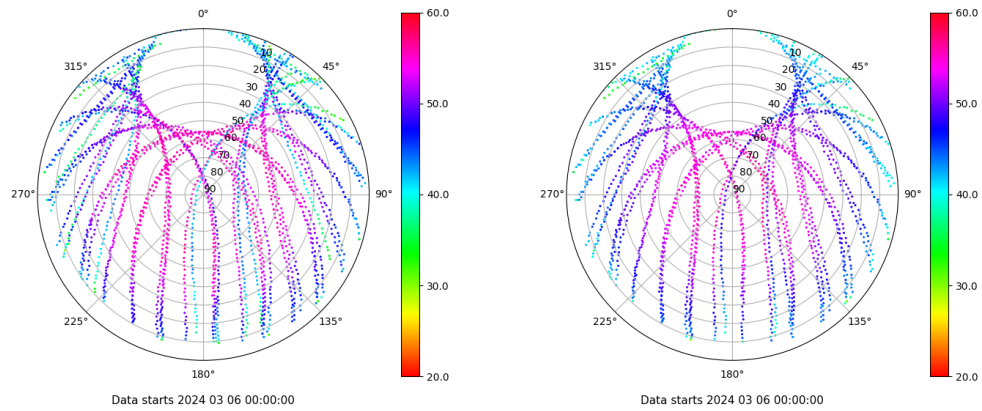
Skyplot for station SPAB. Signal to Noise S1C Data file SPAB00ESP_R_2024066.xtr Skyplot for station SPAB. Signal to Noise S2P Data file SPAB00ESP_R_2024066.xtr
