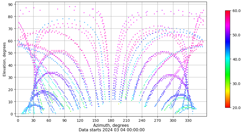
Azimuth-elevation plot for station SPAB. Signal to Noise S1C Data file SPAB00ESP_R_2024064.xtr
