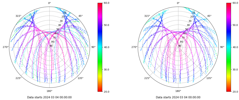
Skyplot for station SPAB. Signal to Noise S1C Data file SPAB00ESP_R_2024064.xtr Skyplot for station SPAB. Signal to Noise S2P Data file SPAB00ESP_R_2024064.xtr
