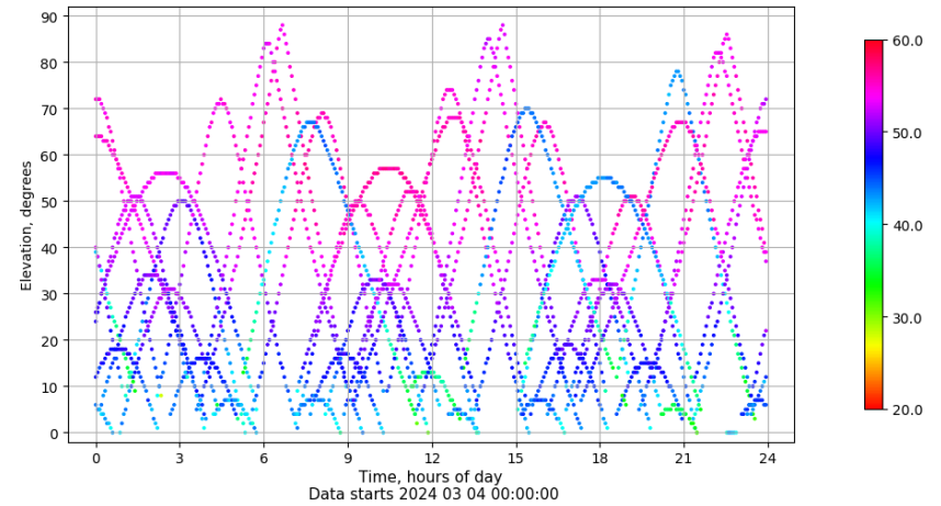
Time-elevation plot for station SPAB. Signal to Noise S1C Data file SPAB00ESP_R_2024064.xtr
