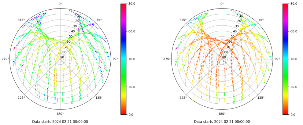
Skyplot for station SPAB. Parameter M1C Data file SPAB00ESP_R_2024052.xtr Skyplot for station SPAB. Parameter M2P Data file SPAB00ESP_R_2024052.xtr
