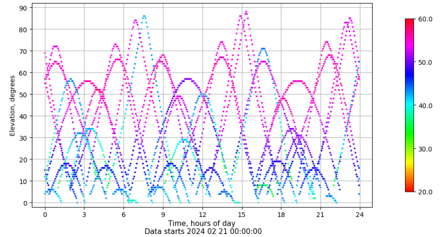
Time-elevation plot for station SPAB. Signal to Noise S1C Data file SPAB00ESP_R_2024052.xtr
