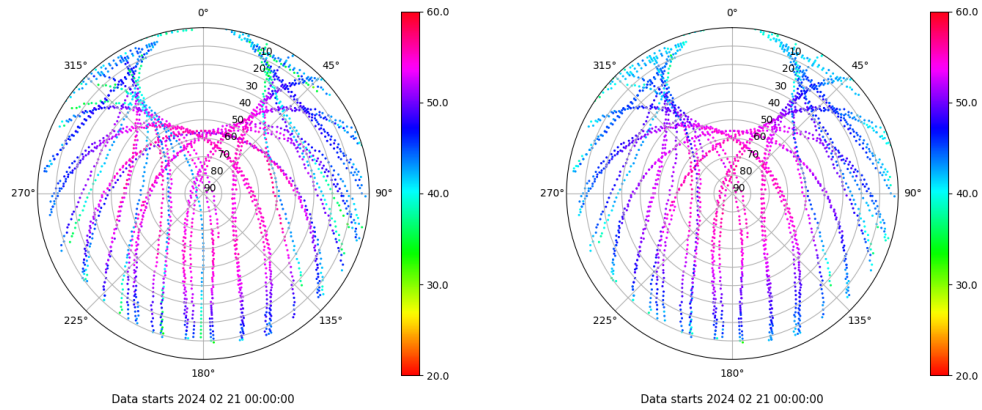
Skyplot for station SPAB. Signal to Noise S1C Data file SPAB00ESP_R_2024052.xtr Skyplot for station SPAB. Signal to Noise S2P Data file SPAB00ESP_R_2024052.xtr
