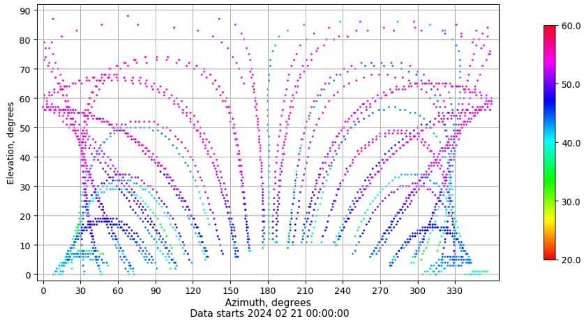
Azimuth-elevation plot for station SPAB. Signal to Noise S1C Data file SPAB00ESP_R_2024052.xtr
