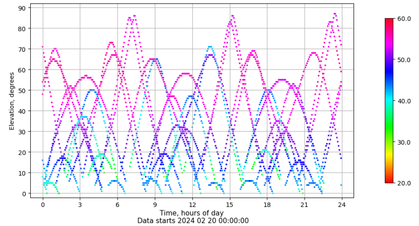
Time-elevation plot for station SPAB. Signal to Noise S1C Data file SPAB00ESP_R_2024051.xtr
