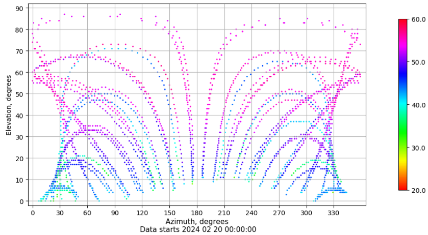
Azimuth-elevation plot for station SPAB. Signal to Noise S1C Data file SPAB00ESP_R_2024051.xtr
