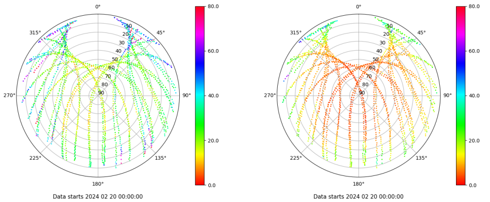
Skyplot for station SPAB. Parameter M1C Data file SPAB00ESP_R_2024051.xtr Skyplot for station SPAB. Parameter M2P Data file SPAB00ESP_R_2024051.xtr
