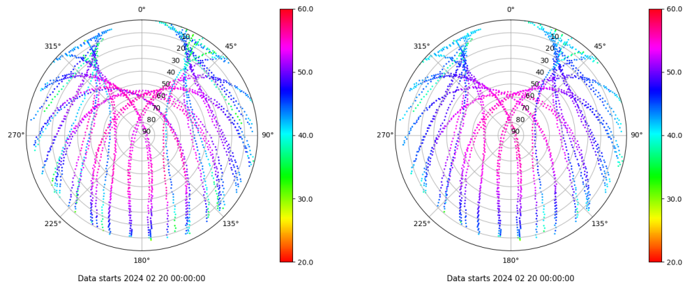
Skyplot for station SPAB. Signal to Noise S1C Data file SPAB00ESP_R_2024051.xtr Skyplot for station SPAB. Signal to Noise S2P Data file SPAB00ESP_R_2024051.xtr
