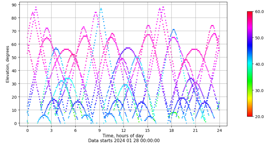
Time-elevation plot for station SPAB. Signal to Noise S1C Data file SPAB00ESP_R_2024028.xtr
