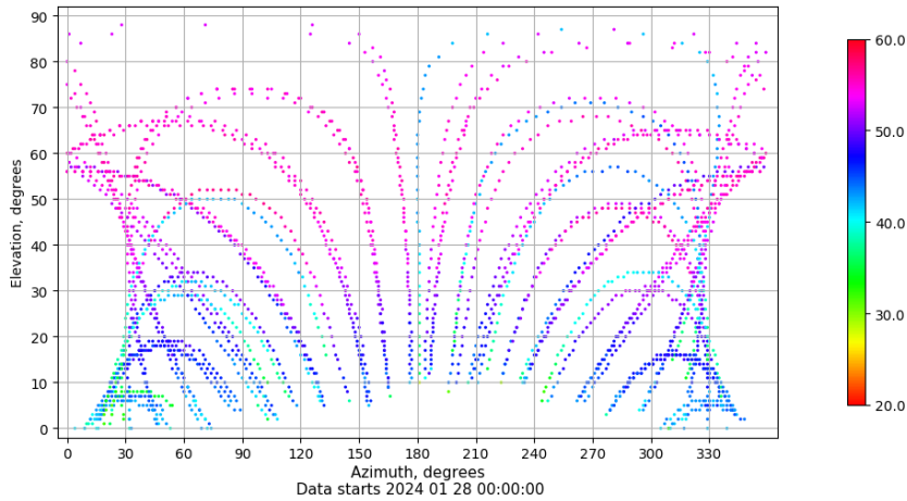
Azimuth-elevation plot for station SPAB. Signal to Noise S1C Data file SPAB00ESP_R_2024028.xtr
