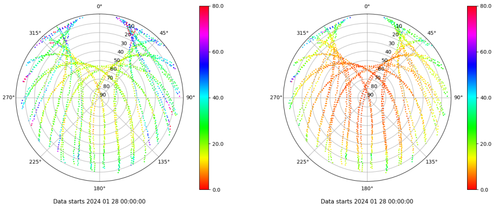
Skyplot for station SPAB. Parameter M1C Data file SPAB00ESP_R_2024028.xtr Skyplot for station SPAB. Parameter M2P Data file SPAB00ESP_R_2024028.xtr
