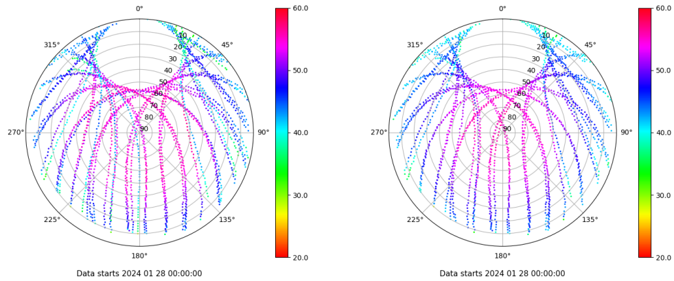
Skyplot for station SPAB. Signal to Noise S1C Data file SPAB00ESP_R_2024028.xtr Skyplot for station SPAB. Signal to Noise S2P Data file SPAB00ESP_R_2024028.xtr
