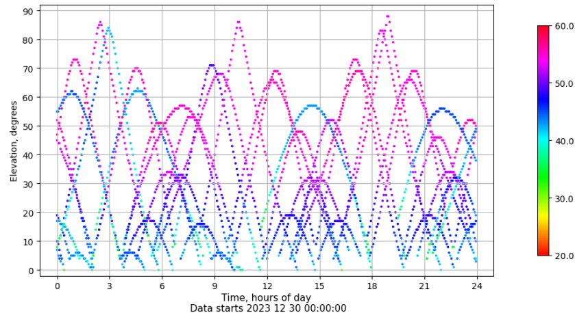
Time-elevation plot for station SPAB. Signal to Noise S1C Data file SPAB00ESP_R_2023364.xtr
