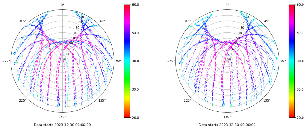
Skyplot for station SPAB. Signal to Noise S1C Data file SPAB00ESP_R_2023364.xtr Skyplot for station SPAB. Signal to Noise S2P Data file SPAB00ESP_R_2023364.xtr
