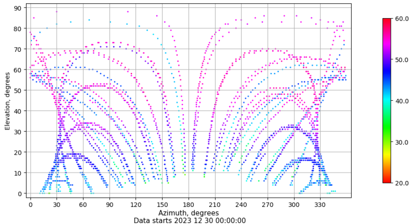
Azimuth-elevation plot for station SPAB. Signal to Noise S1C Data file SPAB00ESP_R_2023364.xtr
