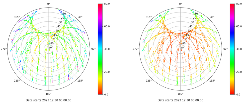
Skyplot for station SPAB. Parameter M1C Data file SPAB00ESP_R_2023364.xtr Skyplot for station SPAB. Parameter M2P Data file SPAB00ESP_R_2023364.xtr
