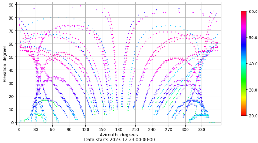
Azimuth-elevation plot for station SPAB. Signal to Noise S1C Data file SPAB00ESP_R_2023363.xtr
