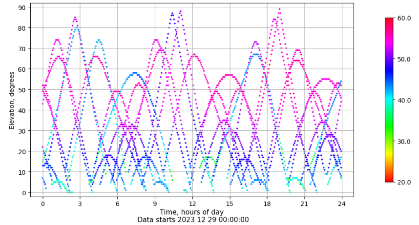
Time-elevation plot for station SPAB. Signal to Noise S1C Data file SPAB00ESP_R_2023363.xtr
