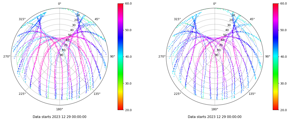
Skyplot for station SPAB. Signal to Noise S1C Data file SPAB00ESP_R_2023363.xtr Skyplot for station SPAB. Signal to Noise S2P Data file SPAB00ESP_R_2023363.xtr
