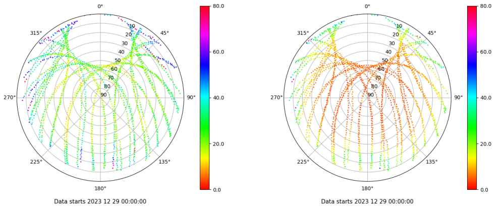
Skyplot for station SPAB. Parameter M1C Data file SPAB00ESP_R_2023363.xtr Skyplot for station SPAB. Parameter M2P Data file SPAB00ESP_R_2023363.xtr
