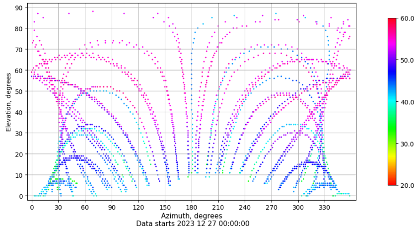
Azimuth-elevation plot for station SPAB. Signal to Noise S1C Data file SPAB00ESP_R_2023361.xtr
