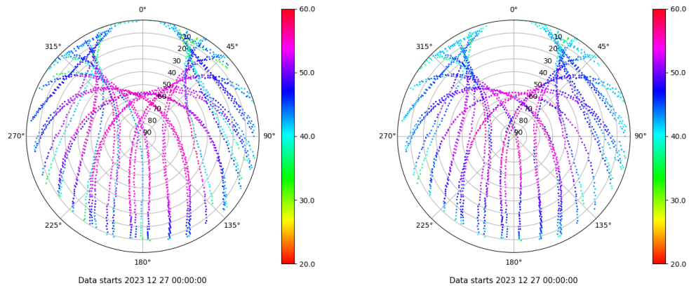
Skyplot for station SPAB. Signal to Noise S1C Data file SPAB00ESP_R_2023361.xtr Skyplot for station SPAB. Signal to Noise S2P Data file SPAB00ESP_R_2023361.xtr
