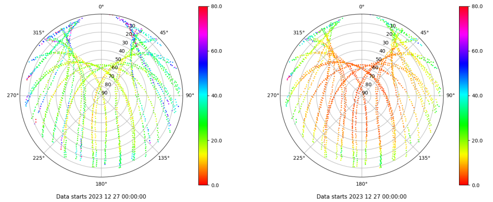
Skyplot for station SPAB. Parameter M1C Data file SPAB00ESP_R_2023361.xtr Skyplot for station SPAB. Parameter M2P Data file SPAB00ESP_R_2023361.xtr
