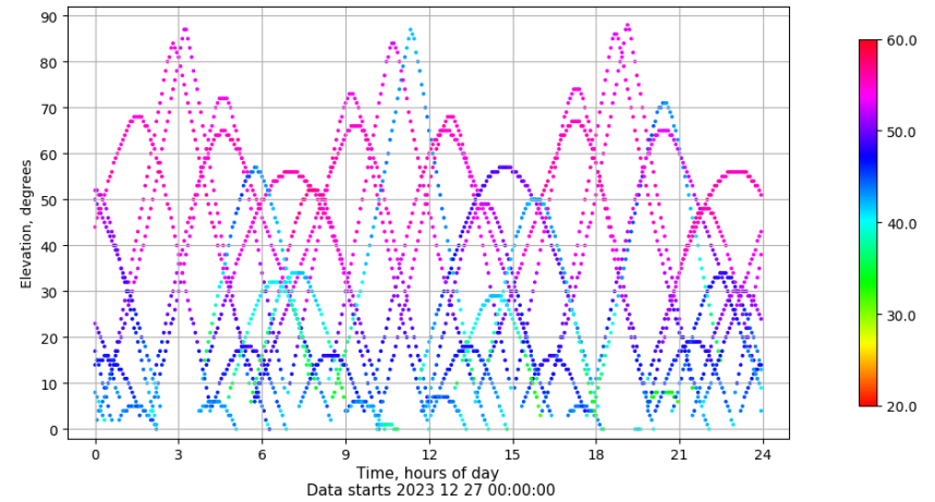
Time-elevation plot for station SPAB. Signal to Noise S1C Data file SPAB00ESP_R_2023361.xtr
